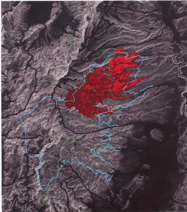
Figure 6 —Calibration of the FARSITE model (in red; 16,686 acres) to a 1-day crown fire run on the northeast head of the Sanford Fire (June 8, 2002; Panguitch, UT). Overlaid on slope are trails (green), roads (black), and the fire perimeter (blue).
