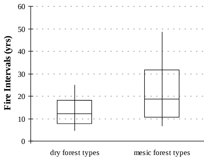
Figure 13. Fire return interval ranges for mesic forest type riparian fire return intervals compared to dry forest type riparian fire return intervals, Baker. Box plots represent, from top to bottom: 90th percentile and 75th percentile exceedance levels, WMPI, 25th percentile and 10th percentile exceedance levels (all percentiles calculated from the Weibull distribution).
