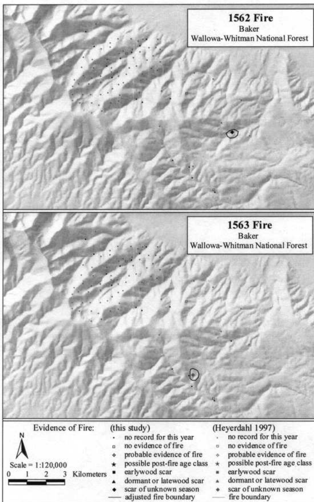
Figure 95. Baker fire maps for 1562 (top) and 1563 (bottom).
