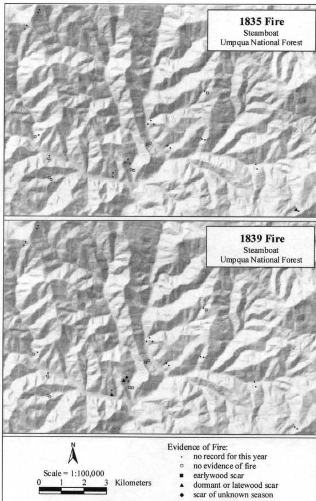
Figure 166. Steamboat fire maps for 1835 (top) and 1839 (bottom).
