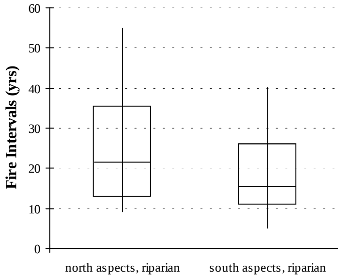
Figure 14. Fire return interval ranges for riparian fire return intervals from north aspects compared to south aspects, Baker. Box plots represent, from top to bottom: 90th percentile and 75th percentile exceedance levels, WMPI, 25th percentile and 10th percentile exceedance levels (all percentiles calculated from the Weibull distribution).
