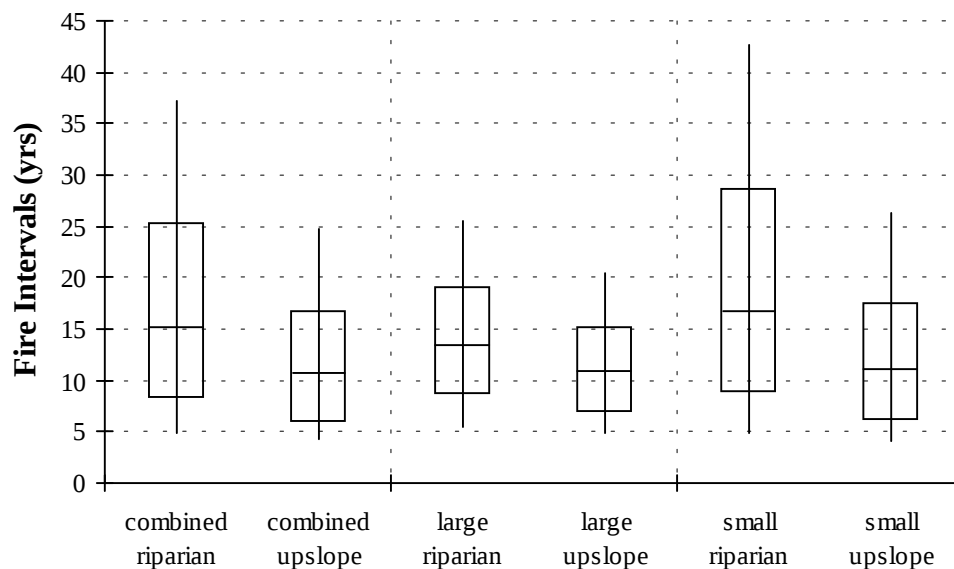
Figure 12. Fire return interval ranges for combined riparian and combined upslope plot categories, large stream riparian and upslope plot categories, and small stream riparian and upslope plot categories, Baker. Box plots represent, from top to bottom: 90th percentile and 75th percentile exceedance levels, WMPI, 25th percentile and 10th percentile exceedance levels (all percentiles calculated from the Weibull distribution).
