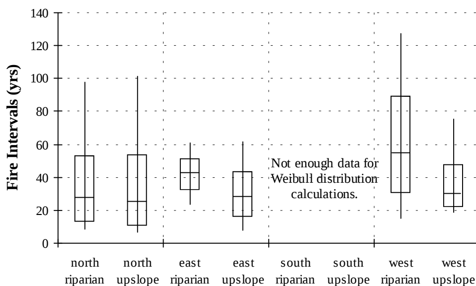
Figure 20. Fire return interval ranges for riparian and upslope fire return intervals from north, east, south and west aspects, Steamboat. Box plots represent, from top to bottom: 90th percentile and 75th percentile exceedance levels, WMPI, 25th percentile and 10th percentile exceedance levels (all percentiles calculated from the Weibull distribution). There were not enough fire return intervals in the south-facing riparian and upslope fire return interval categories to determine WMPIs or confidence intervals.
