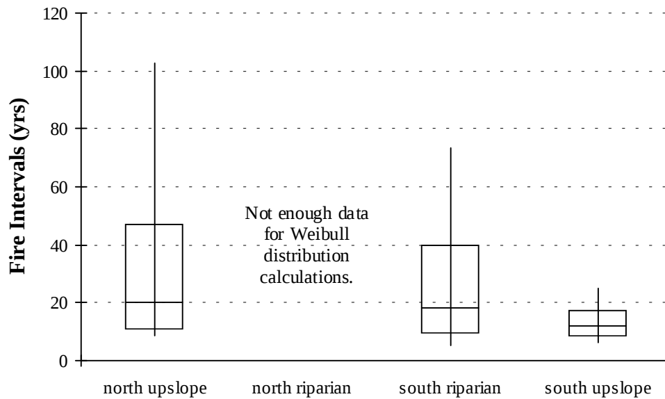
Figure 16. Fire return interval ranges for riparian and upslope fire return intervals from north- and south-facing aspects in the mid-elevational range of the Marble Creek drainage, Baker. Box plots represent, from top to bottom: 90th percentile and 75th percentile exceedance levels, WMPI, 25th percentile and 10th percentile exceedance levels (all percentiles calculated from the Weibull distribution). There were not enough fire return intervals in the north-facing riparian fire return interval category to determine a WMPI or confidence intervals.
