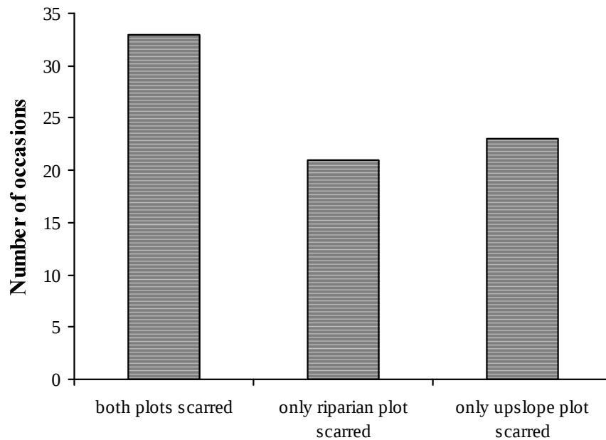
Figure 23. The number of occasions where fires scarred both riparian and upslope plots, compared to occasions where fires scarred only the riparian plot or only the upslope plot, Steamboat.
