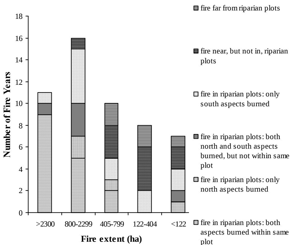
Figure 17. Number of fires that burned in Baker riparian plots, categorized by fire extent size classes and the aspect within the riparian plot.
