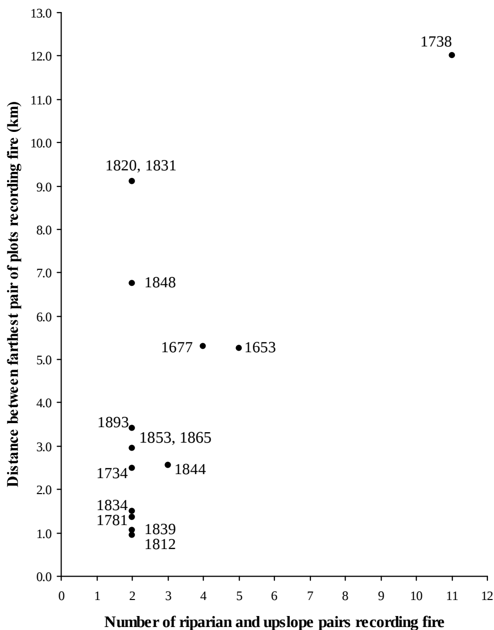
Figure 22. Fire years between 1650 and 1900 showing evidence of fire in two or more pairs of plots, and the distance between the two farthest plots recording each fire, Steamboat.
