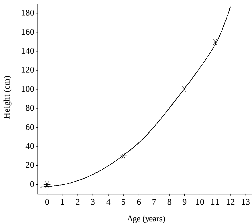
Figure 8. Age versus height curve for Douglas-fir, extrapolated from McArdle and Meyer (1930).
