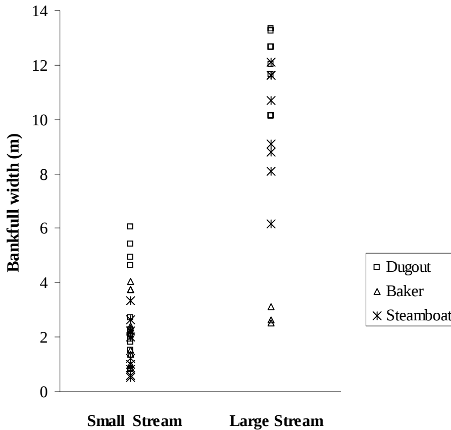
Figure 3. Bankfull widths categorized by stream size for all of the riparian plots in each of the three study areas.
