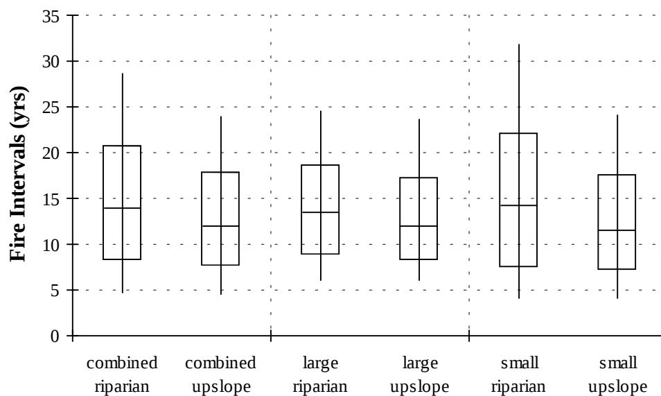
Figure 9. Fire return interval ranges for combined riparian and combined upslope plot categories, large stream riparian and upslope plot categories, and small stream riparian and upslope plot categories, Dugout. Box plots represent, from top to bottom: 90th percentile and 75th percentile exceedance levels, WMPI, 25th percentile and 10th percentile exceedance levels (all percentiles calculated from the Weibull distribution).
