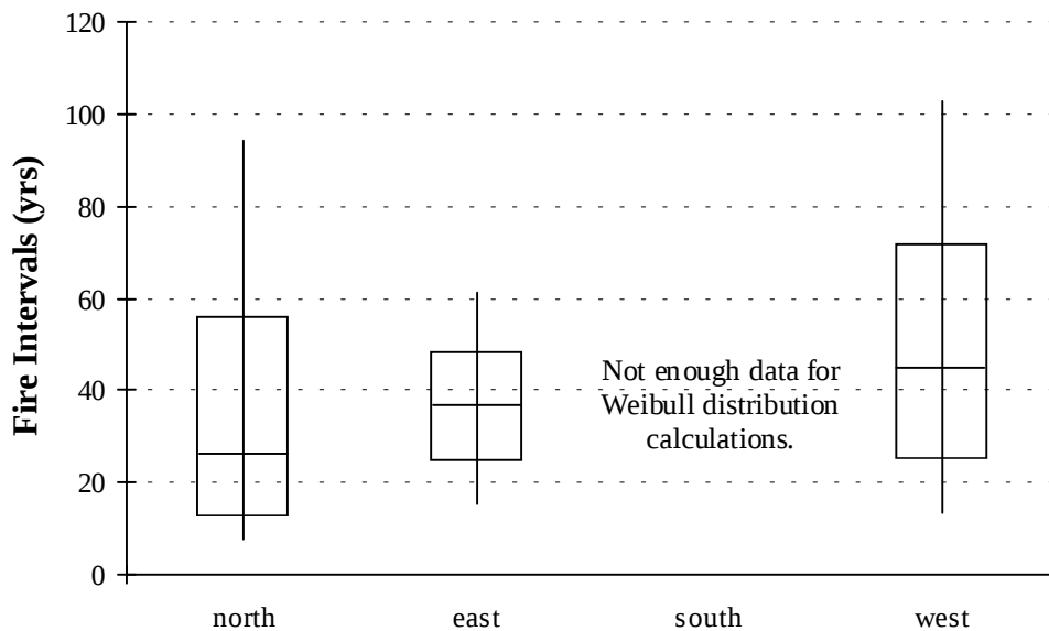
Figure 19. Fire return interval ranges for combined riparian and upslope fire return intervals from north, east, south and west aspects, Steamboat. Box plots represent, from top to bottom: 90th percentile and 75th percentile exceedance levels, WMPI, 25th percentile and 10th percentile exceedance levels (all percentiles calculated from the Weibull distribution). There were not enough fire return intervals in the south-facing fire return interval category to determine a WMPI or confidence intervals.
