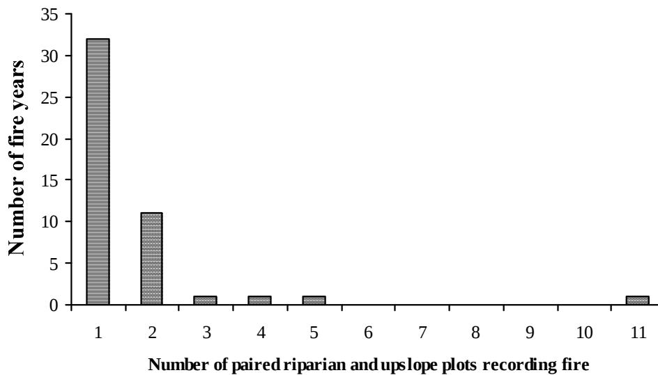
Figure 21. Number of fire years in the Steamboat study area between 1650 and 1900, in relation to the number of paired riparian and upslope plots recording each fire.
