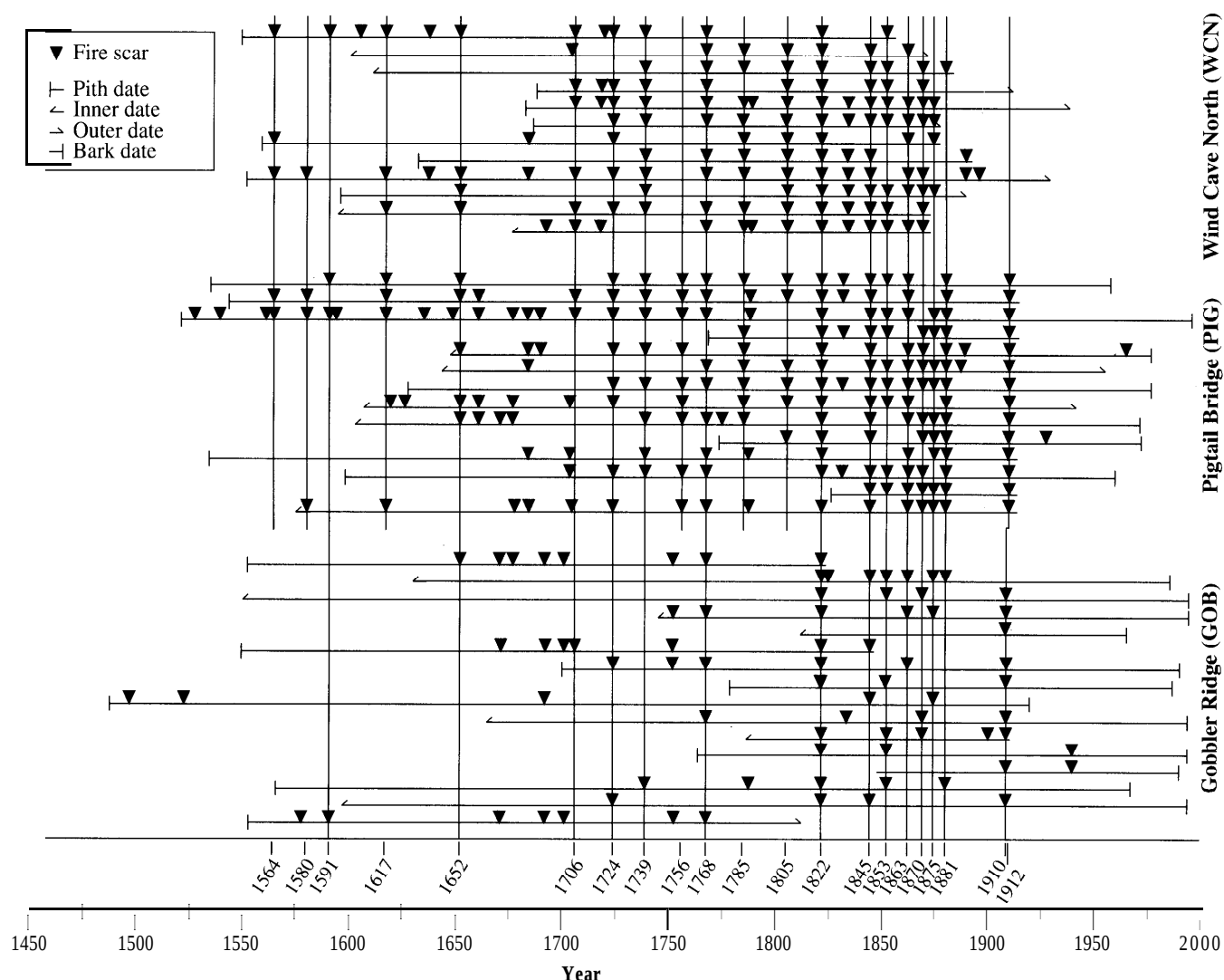
FIGURE 3. Fire chronologies for Wind Cave National Park sites. Time spans of individual trees are represented by horizontal lines, with fire scars noted by triangles at the dates they were recorded. Dates at the bottom of the fire chronologies are those years when fire scars were recorded at more than one site, except for 1910 and 1912 which were recorded only at sites GOB and PIG, respectively.
