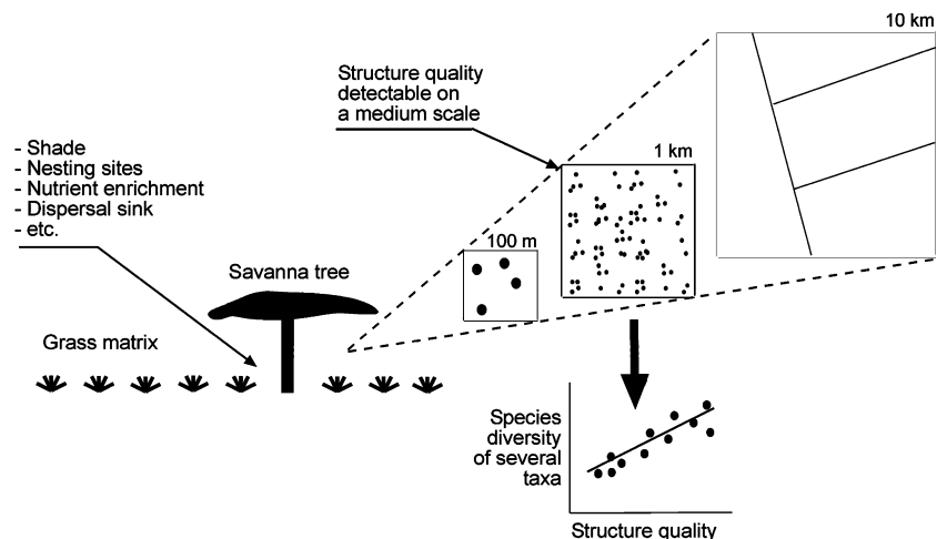
Figure 4 Tree savannas are a typical keystone structure ecosystem. A wide array of species groups (e.g. arthropods, birds or mammals) depend on trees as a food resource, shelter or nesting site. Consequently, overall species diversity is strongly linked to the quality of this structure. The quality, e.g. the proportion of large, solitary trees is detectable on a medium spatial scale: if the scale is too small distinction between degraded savanna sites and intact savanna with high structural diversity is difficult to quantify, if the scale is too large, large-scale landscape components such as land-use patterns may yield biased results.
