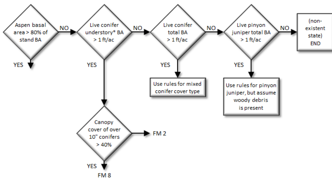
Figure 4.17.2 - Logic for modeling fire at "low" fuel loads in the TT-FFE variant.
