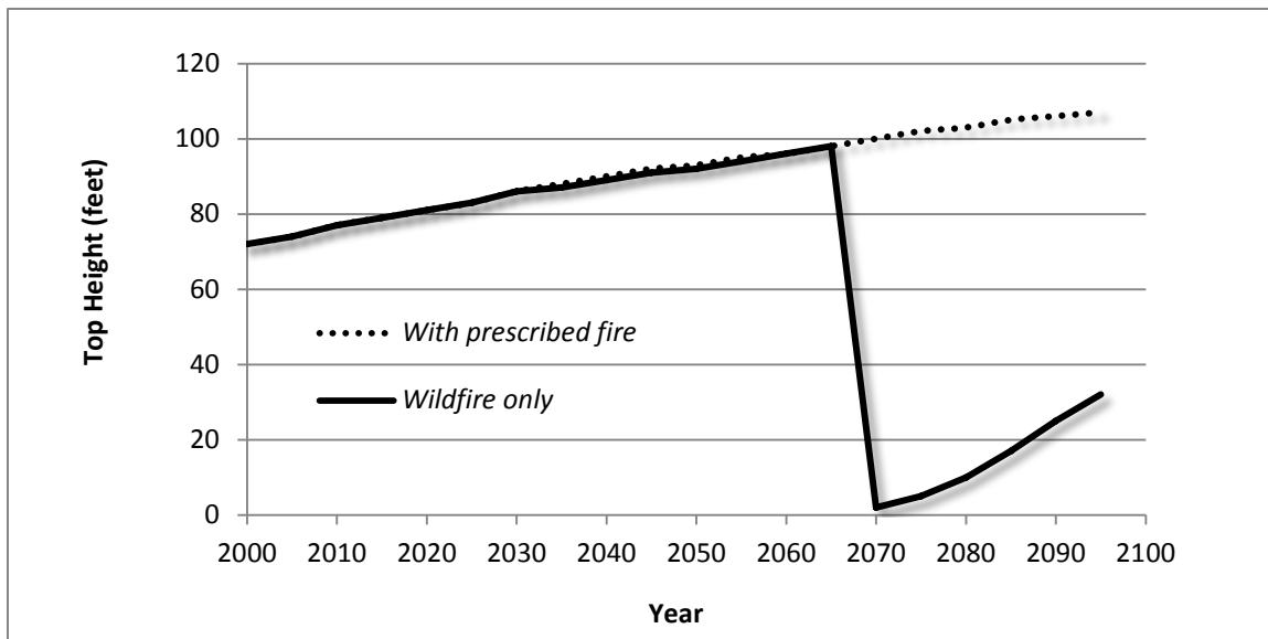
Figure 1.2.8 - Top height is the average height of the largest 40 trees per acres. The scenarios provide similar top heights until wildfire.
