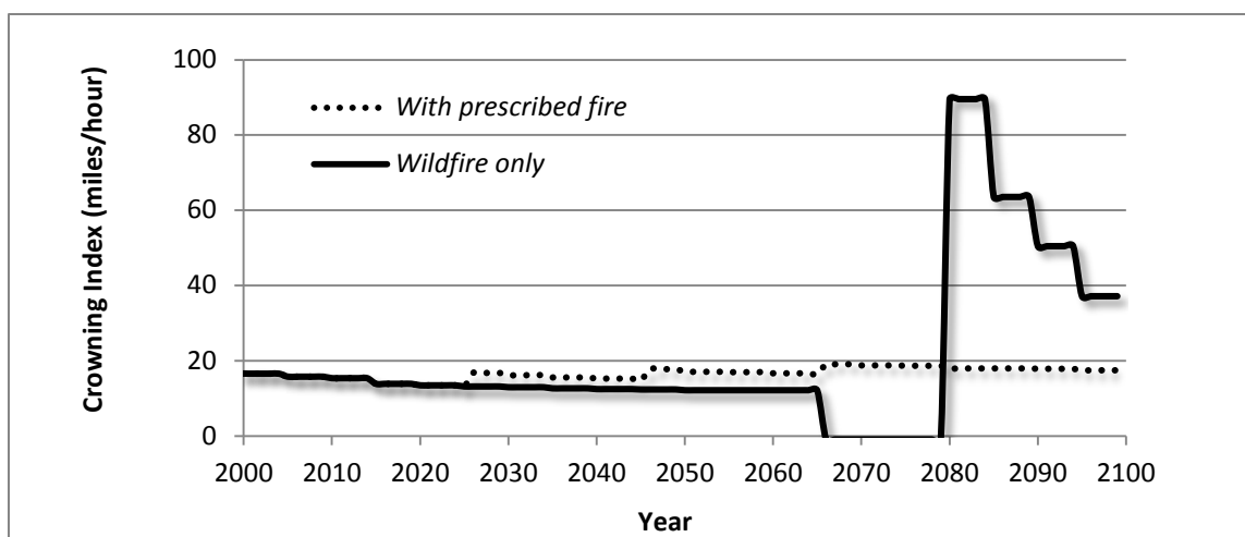
Figure 1.2.3 – The crowning index is one measure of crown fire hazard and is the windspeed needed to support an active crown fire. In this case, the crowning index is higher (less hazardous) when prescribed fire is included. In the wildfire only simulation, the crowning index increases after the wildfire as a result of the mortality and fuel consumption.
