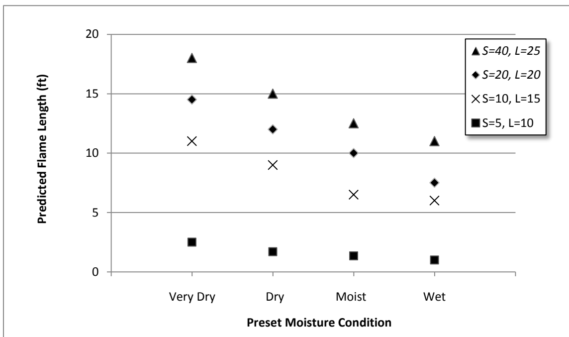
Figure 2.5.1 - Example flame lengths for each of the predefined moisture conditions for four different combinations of small ( S < 3'' ) and large ( L > 3'' ) fuel amounts (in tons/acre). Other factors being equal, the flame lengths decrease as moisture levels increase.
