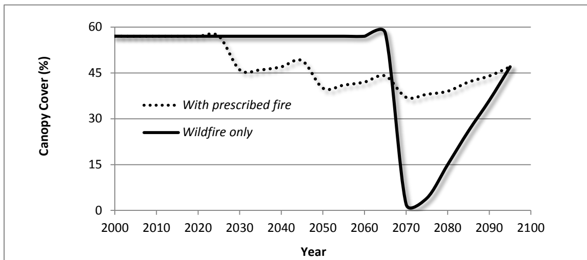
Figure 1.2.6 - Canopy cover is a key variable used in habitat assessments. The prescribed fires caused a steady reduction of this variable while the Wildfire only scenario provided significant cover until the wildfire of 2065.
