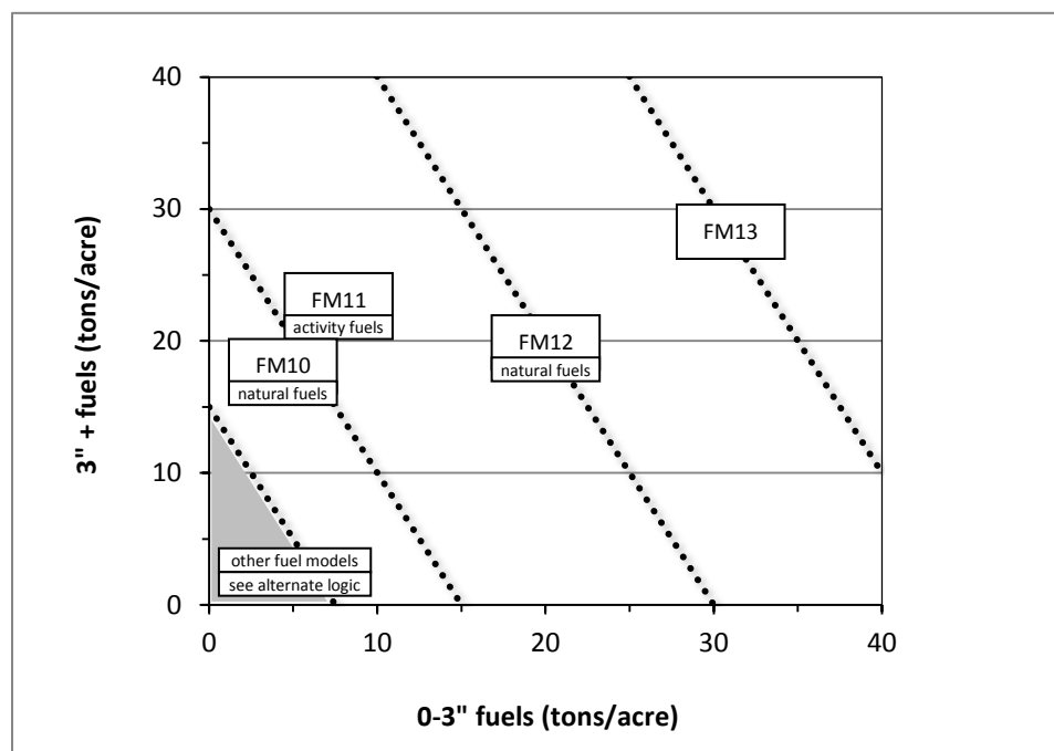
Figure 4.4.2 - If large and small fuels map to the shaded area, candidate fuel models are determined using the logic shown in Table 4.4.15. Otherwise, flame length based on distance between the closest fuel models, identified by the dashed lines, and on recent management (see section 2.4.8 for further details).
