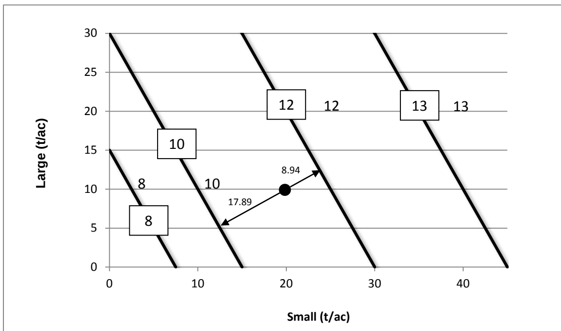
Figure 2.4.4 - An example of dynamic fuel modeling, based on large and small woody surface fuel. The lines here correspond to fuel models for natural fuel in closed stands for many habitat types, with the fuel model number shown on the line. The point shown below here will result in an interpolation using Fuel Models 10 and 12, as described in the text.
