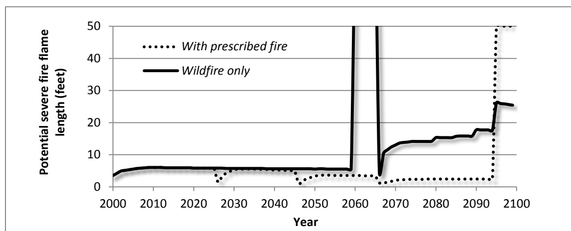
Figure 1.2.2 - The potential fire flame length for severe burning conditions is illustrated with both scenarios. The With prescribed fire scenario has a much lower potential flame length in this example until the end of the simulation where it jumps to 50 feet.
