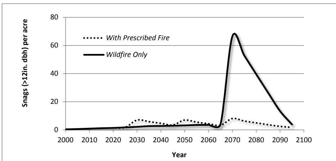
Figure 1.2.5 - The number of large snags per acre for the two scenarios.
