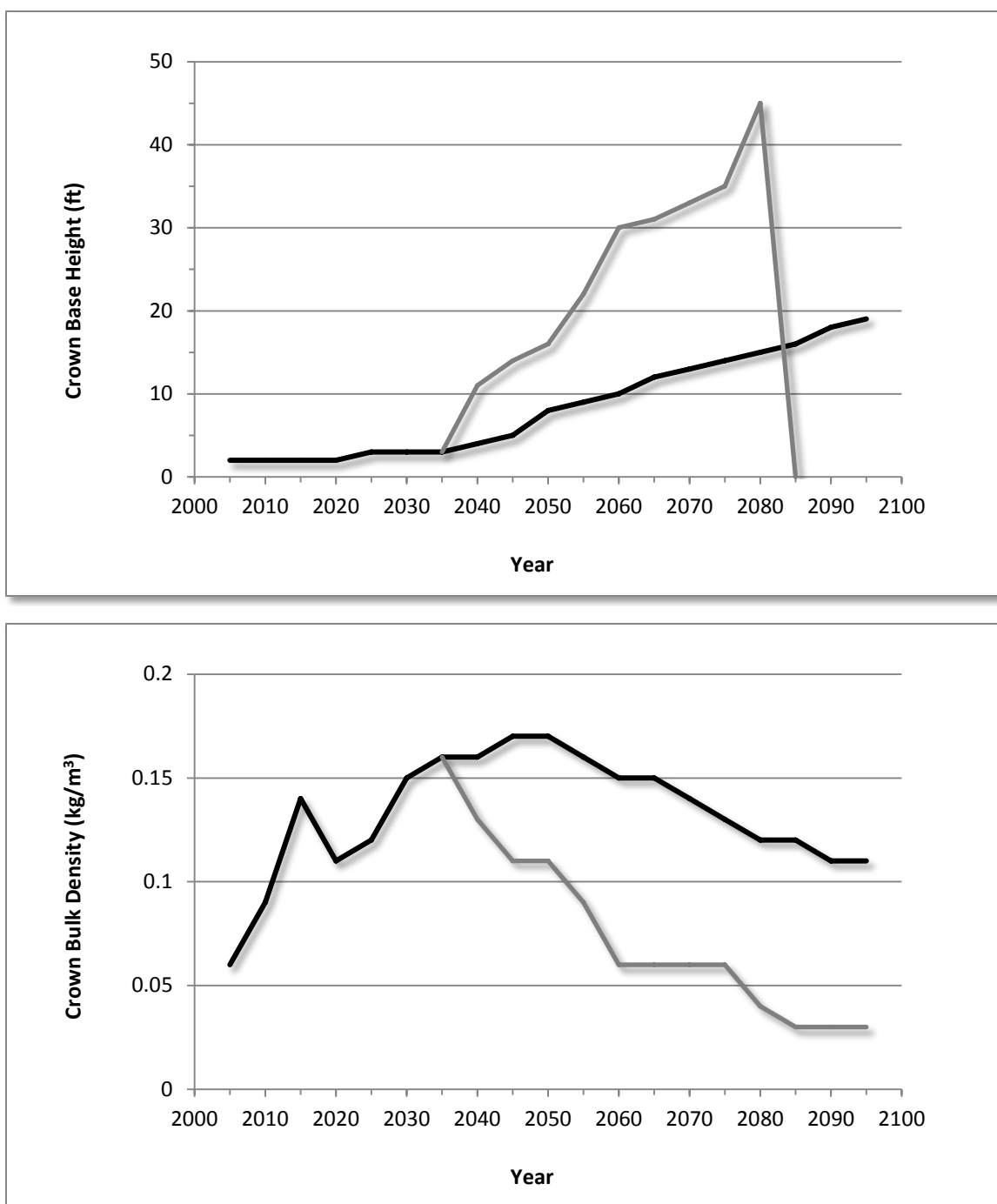
Figure 2.5.10 - Canopy base height and bulk density under different management scenarios. A mixed-conifer stand is established at the beginning of the simulation (thick line). In one scenario this stand is repeatedly thinned from below (thin line). The canopy fuel is independent of whether the harvested material is removed or left in the stand.
