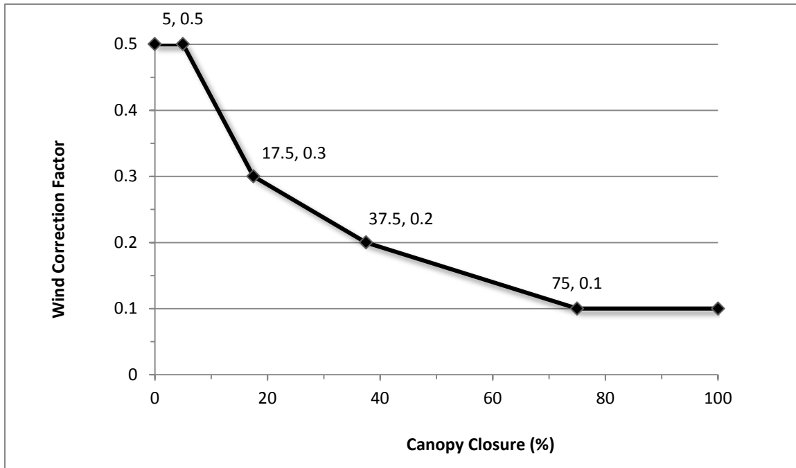
Figure 2.5.2 - The correction factors used to calculate mid-flame wind speed from wind at 20 feet above the ground or the top of vegetation
