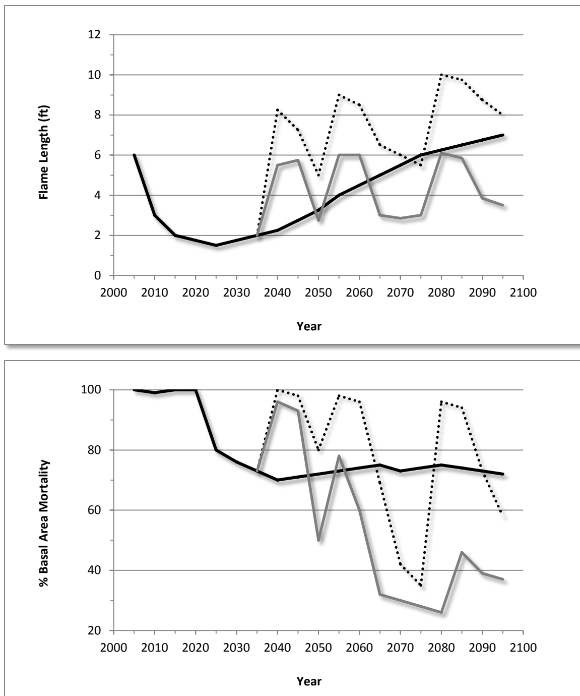
Figure 2.5.9 - Potential flame length and mortality in a stand under three management scenarios. The stand is established at the beginning of the run. In one scenario no treatment was applied (thick line). In two scenarios the stand was thinned from below (in 2040, 2055, and 2080). In one scenario, the harvested material was left on the ground causing an increase in surface fuels, and thus in potential flame length and mortality (dotted line) and in the other scenario it was all removed (thin line). Even when activity fuels are removed, flame length increases temporarily after thinning because reductions in canopy cover cause an increase in mid-flame wind speed.
