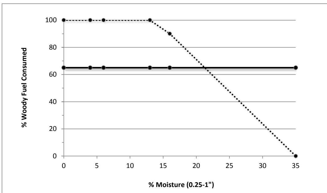
Figure 2.5.7 - Predicted fuel consumption for 1 to 3 inches woody fuel for different moisture levels. The points on the graph indicate the values at the four default fuel moisture conditions. The solid line is for the naturally occurring fuel, while the dotted line is for fuel resulting from management activities. Notice that the consumption of larger fuel depends on the moisture values of the smaller fuel.
