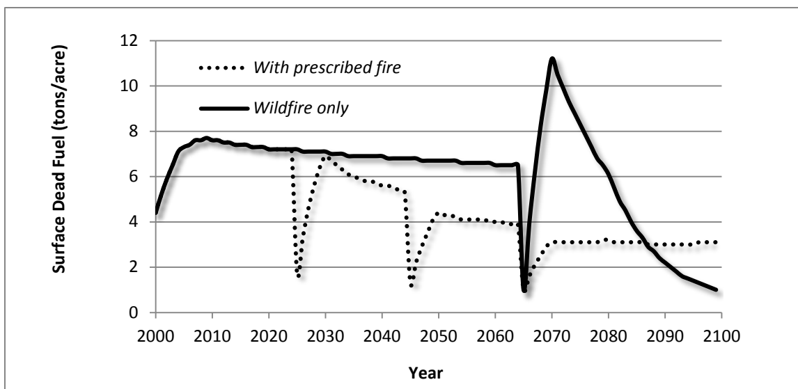
Figure 1.2.4 - Surface fuel loads are of interest to fuel managers. To wildlife and vegetation managers, this variable measures down woody debris. For the Wildfire only scenario, the model predicts surface fuel decomposition exceeds accumulation after the initial accumulation.
