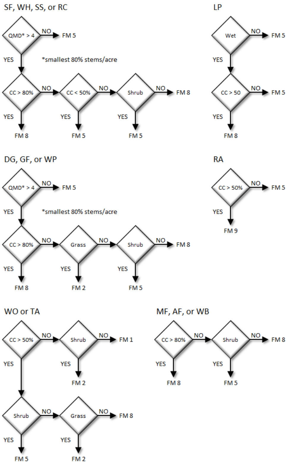
Figure 4.14.2 - Fuel models for the PN-FFE variant.
