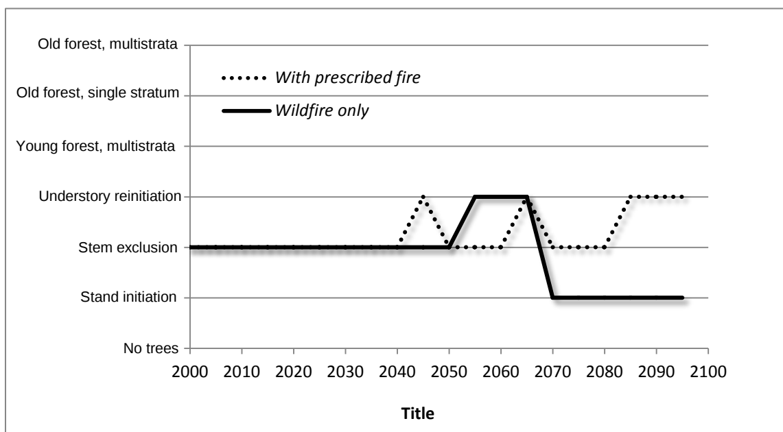
Figure 1.2.7 - Stand structure is classified by FVS (Crookston and Stage, 1999) and plotted here for each scenario. After the 2065 wildfire, the With prescribed fire scenario maintains later successional stages when compared to Wildfire only .
