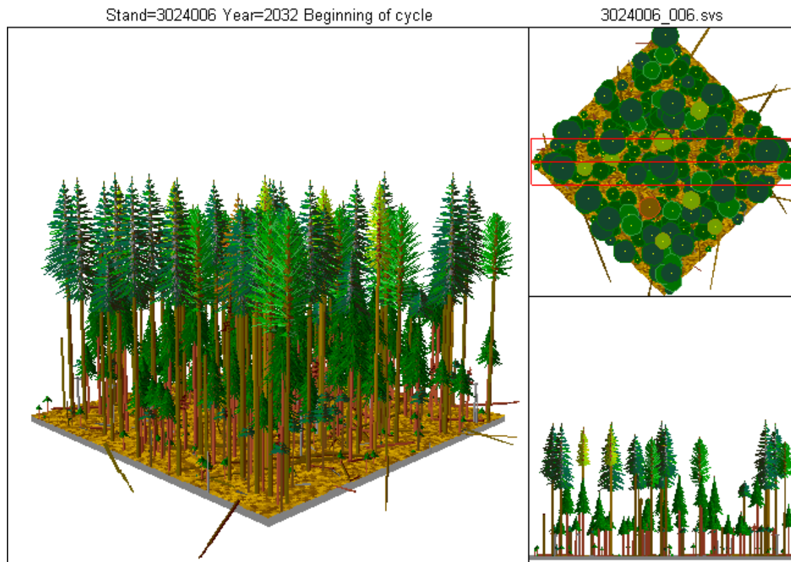
Figure A.3.2 - Example stand 3024006 shown at year 2032 without management using SVS (McGaughey 1997; http://www.fs.fed.us/pns/svs ).
