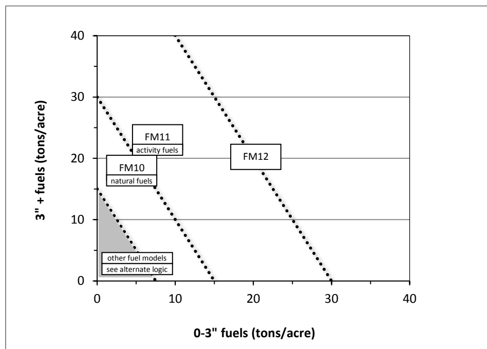
Figure 4.17.1 - If large and small fuels map to the shaded area, candidate fuel models are determined using the logic shown in figure 4.10.2. Otherwise, flame length based on distance between the closest fuel models, identified by the dashed lines, and on recent management (see section 2.4.8 for further details).
