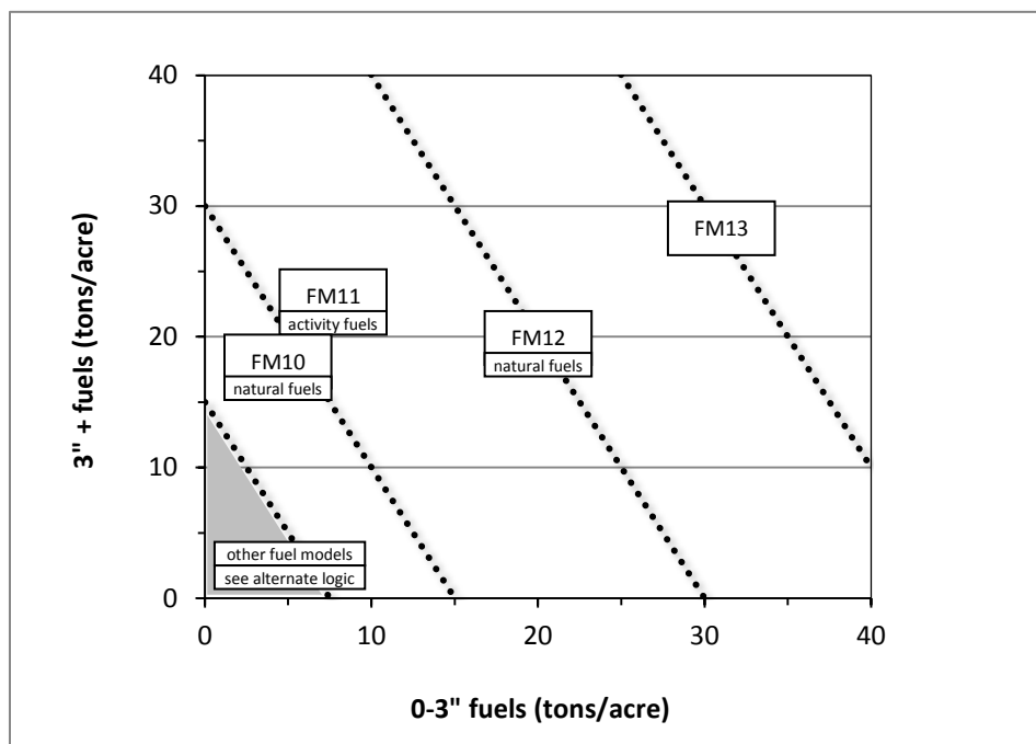
Figure 4.20.2 - If large and small fuels map to the shaded area, candidate fuel models are determined using the logic shown in table 4.82. Otherwise, flame length based on distance between the closest fuel models, identified by the dashed lines, and on recent management (see section 2.4.8 for further details).
