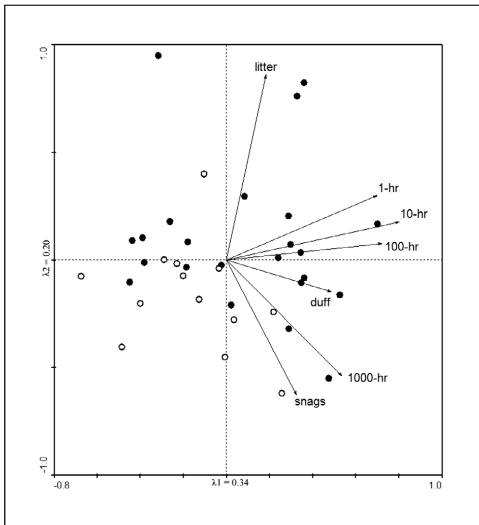
Figure 3. PCA diagram for fuel composition at Lava Cast Forest. Dark circles represent plots infested with mistletoe; open circles represent non-infested plots. The first axis represents a gradient of 1-, 10-, and 100-hr fuels; the second axis 1000-hr and litter.
