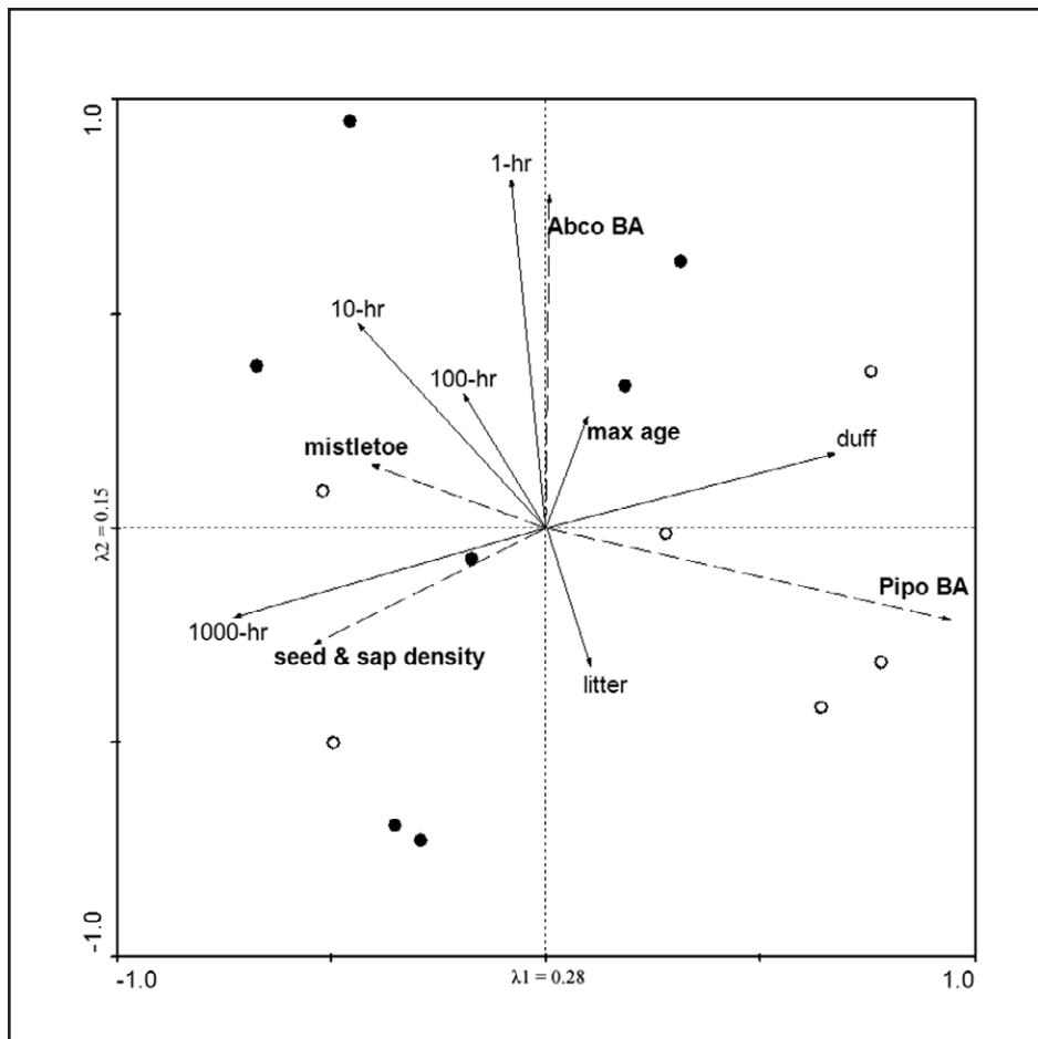
Figure 2. RDA diagram for Crater Lake plots. Dark circles represent plots infested with mistletoe; open circles represent non-infested plots. Environmental variables are indicated by bold text and dashed vectors. Fuel variables are indicated by solid vectors.
