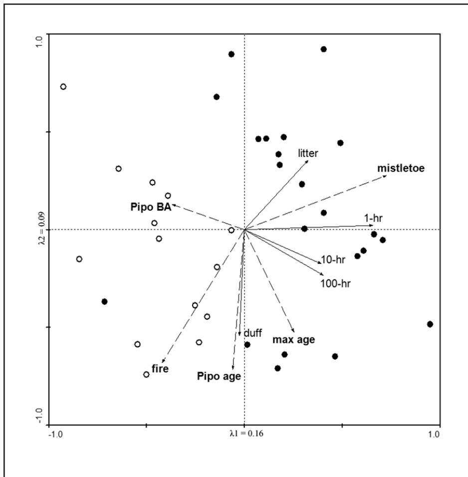
Figure 4. RDA results for Lava Cast Forest plots. Dark circles represent plots infested with mistletoe; open circles represent non-infested plots. Stand structure variables are indicated by bold text and dashed vectors. Fuel variables are indicated by solid vectors. Pipo = ponderosa pine; BA = basal area; fire = years since last fire.
