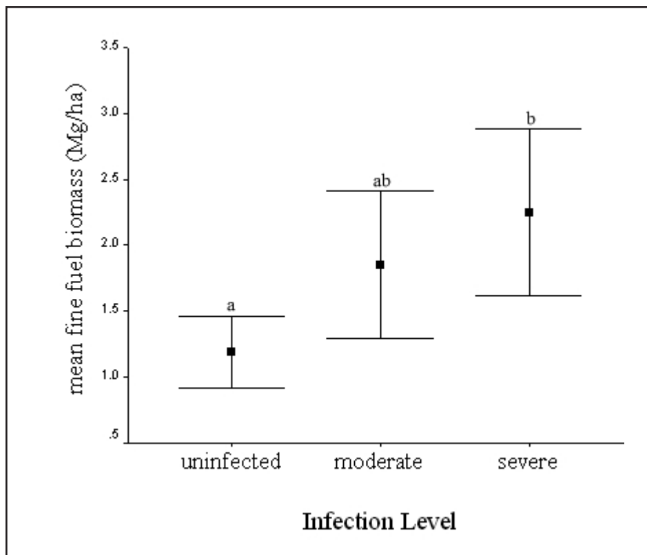
Figure 5. Sum of fine woody fuel loads (1-, 10- and 100-hr fuels; mean \pm 1 SE) by dwarf mistletoe infection level (moderate = mean plot DMR 3 or 4; severe = mean plot DMR 5 or 6) for Lava Cast Forest, Oregon. Different letters (a or b) denote statistically different means determined by one-way ANOVA ( P \leq 0.05 ).
