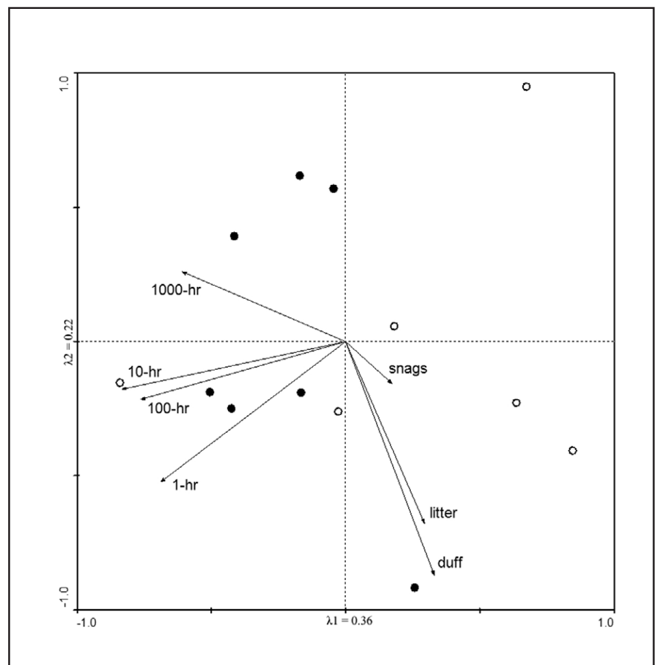
Figure 1. PCA diagram for fuel composition in Crater Lake plots. Dark circles represent plots infested with mistletoe; open circles represent non-infested plots. The first axis represents a gradient of 1-, 10-, and 100-hr fuels; the second axis 1000-hr fuels and duff.
