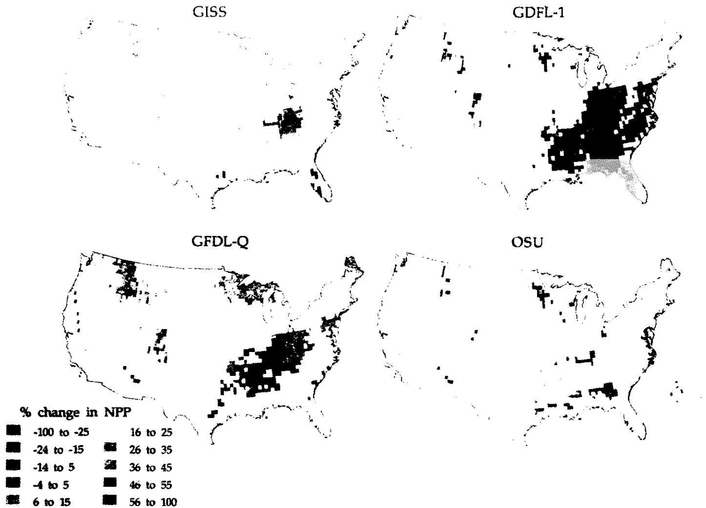
Figure 2.6.—Spatial comparison of the responses in annual net primary production (NPP) between contemporary climate at 355 ppmv CO 2 and the various GCM climates at 625 ppmv CO 2 as predicted by the Terrestrial Ecosystem Model for the 1443 grid cells (0.5° latitude by 0.5° longitude) that describe the historical range of temperate forests in the United States (see fig. 2.1).
