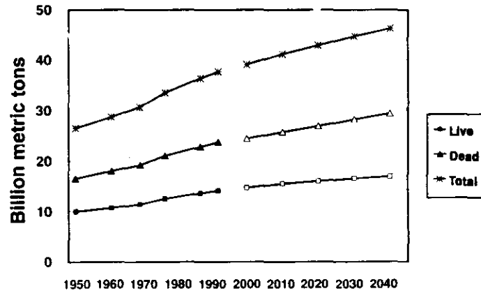
Figure 4.3.—Carbon storage in live (tree and understory) and dead (soil and forest floor) organic matter, conterminous U.S. forests, 1952-2040.
