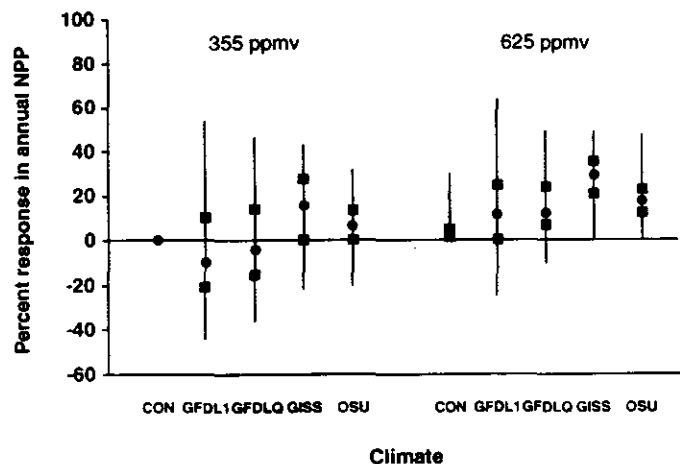
Figure 2.5.—The distributions of response of annual net primary production (NPP) between contemporary climate at 355 ppmv \text{CO}_2 and the various GCM climates at 355 ppmv \text{CO}_2 (left side of figure) and contemporary and GCM climates at 625 ppmv \text{CO}_2 (right side of figure) as predicted by the Terrestrial Ecosystem Model for the 1443 grid cells ( 0.5^\circ latitude by 0.5^\circ longitude) that describe the historical range of temperate forests in the United States (see fig. 2.1). Abbreviations for climates are as follows: CON, contemporary; GFDL1, Geophysical Fluid Dynamics Laboratory 1; GFDLQ, Geophysical Fluid Dynamics Laboratory Q; GISS, Goddard Institute for Space Studies; and OSU, Oregon State University. Circles identify the median and squares the 25th and 75th percentiles of the distributions. Solid lines delineate the range.
