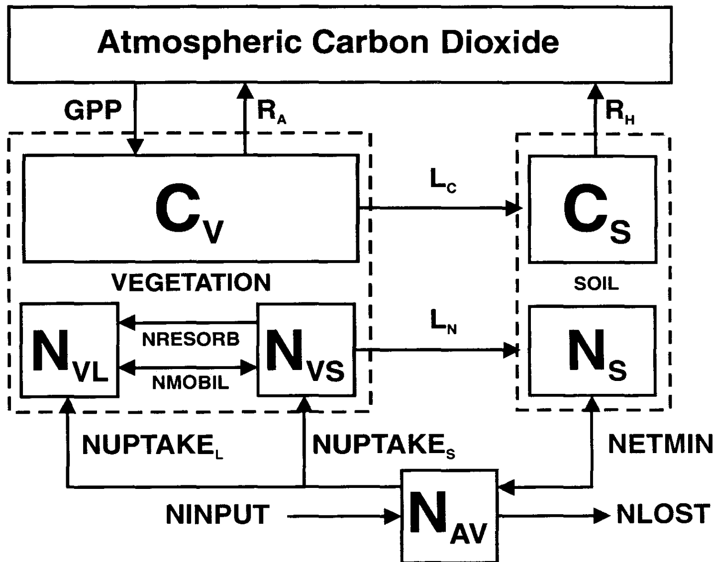
Figure 2.4.—The Terrestrial Ecosystem Model (TEM). The state variables are: carbon in the vegetation (C V ); structural nitrogen in the vegetation (N VS ); labile nitrogen in the vegetation (N VL ); organic carbon in soils and detritus (C S ); organic nitrogen in soils and detritus (N S ); and available soil inorganic nitrogen (N AV ). Arrows show carbon and nitrogen fluxes: GPP, gross primary productivity; R A , autotrophic (plant) respiration; R H , heterotrophic respiration; L C , litterfall carbon; L N , litterfall nitrogen; NUPTAKE S , nitrogen uptake into the structural nitrogen pool of the vegetation; NUPTAKE L , nitrogen uptake into the labile nitrogen pool of the vegetation; NRESORB, nitrogen resorption from dying tissue into the labile nitrogen pool of the vegetation; NMOBIL, nitrogen mobilized between the structural and labile nitrogen pools of the vegetation; NETMIN, net nitrogen mineralization of soil organic nitrogen; NINPUT, nitrogen inputs from outside the ecosystem; and NLOST, nitrogen losses from the ecosystem.
