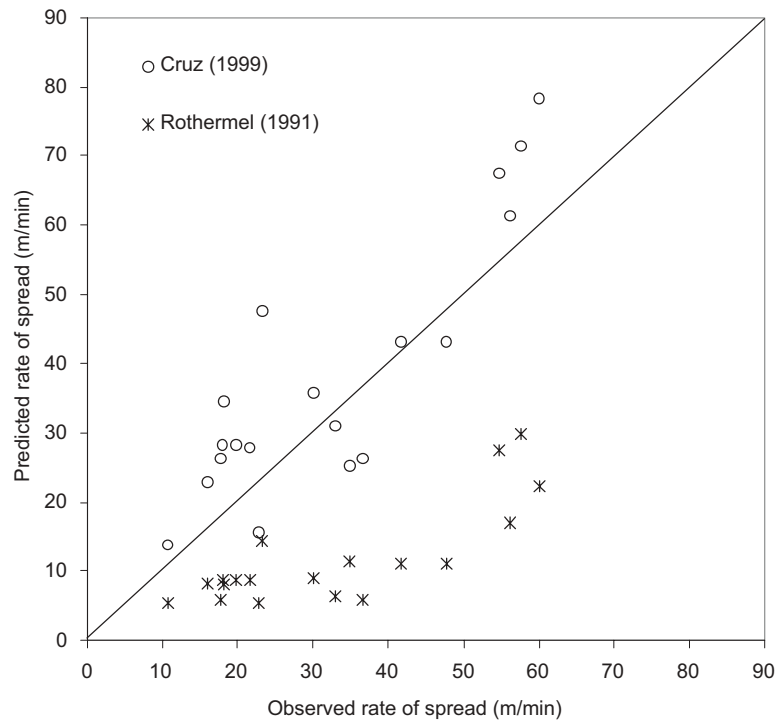
Figure 1 —Plot of observed versus predicted rate of spread of crown fires in the Rothermel (1991) and Cruz (1999) crown fire spread models.
