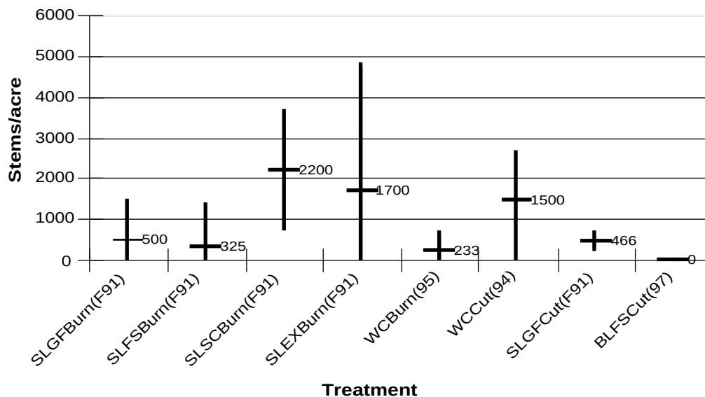
Figure 2 —Mean and one standard deviation for stem densities of aspen suckers >10 ft in height at time of sampling.
