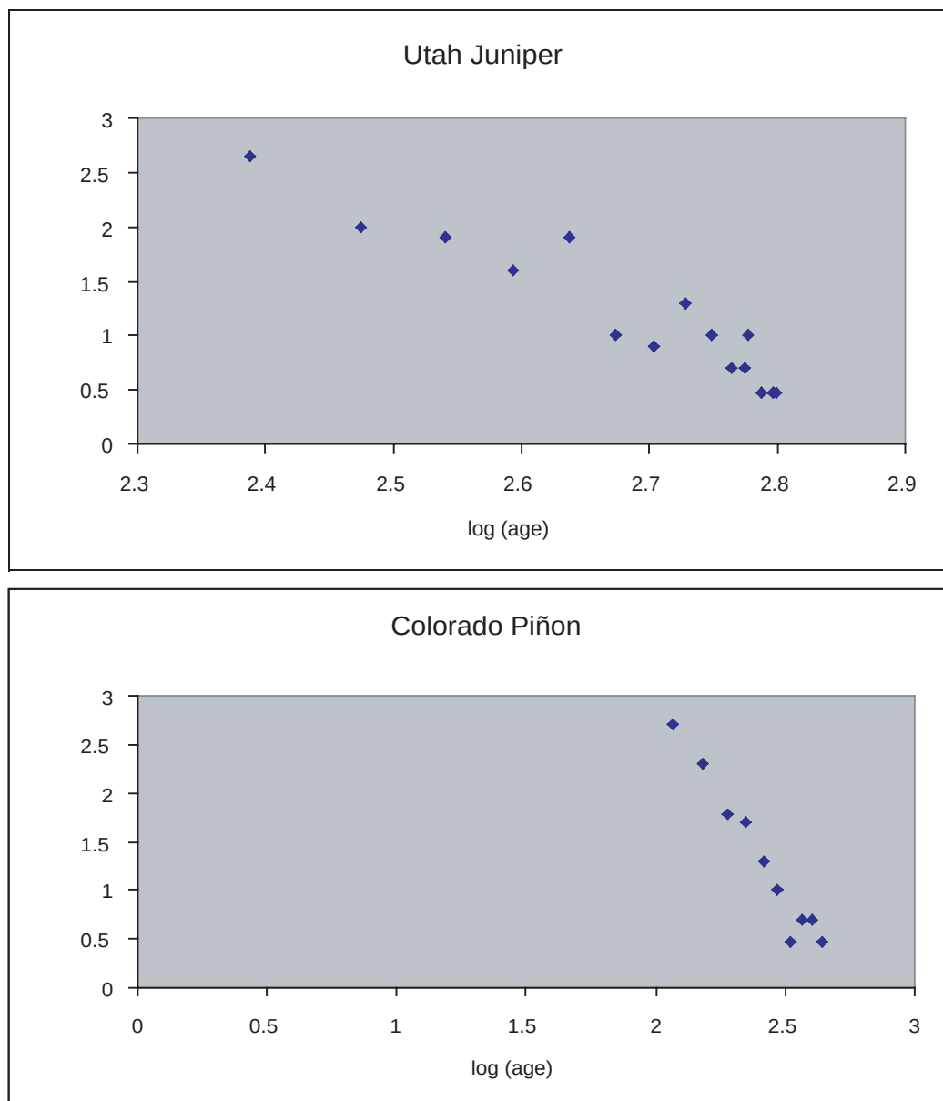
Figure 4 —A plot of \log(\text{stems/ha}) vs. \log(\text{tree age}) for a stand of dense piñon-juniper forest at the southern end of Mesa Verde National Park. The linear relationship for Juniperus osteosperma (a) and for Pinus edulis (b) indicates that both tree species have an approximately stationary age structure of the kind that is associated with stable, old-growth forests (Leak 1975).
