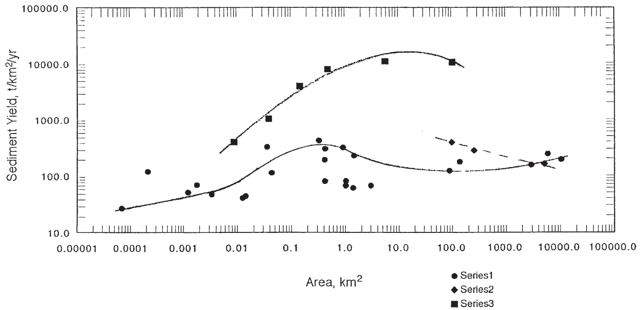
Figure 14 —Sediment yield as a function of drainage-basin area for Walnut Gulch/San Pedro River Basin (series 1), with additional data and lines of relation for the San Simon Creek Basin (series 2, dashed line), and a condition of accelerated erosion in the Walnut Gulch Basin (series 3). Relation lines are visual interpretations of best fit.
