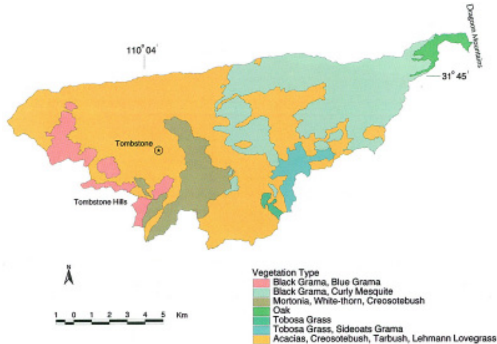
Figure 6 —Distribution of dominant vegetation species, as vegetation types, in the Walnut Gulch Experimental Watershed (unpublished map, courtesy of S. N. Miller, ARS).
