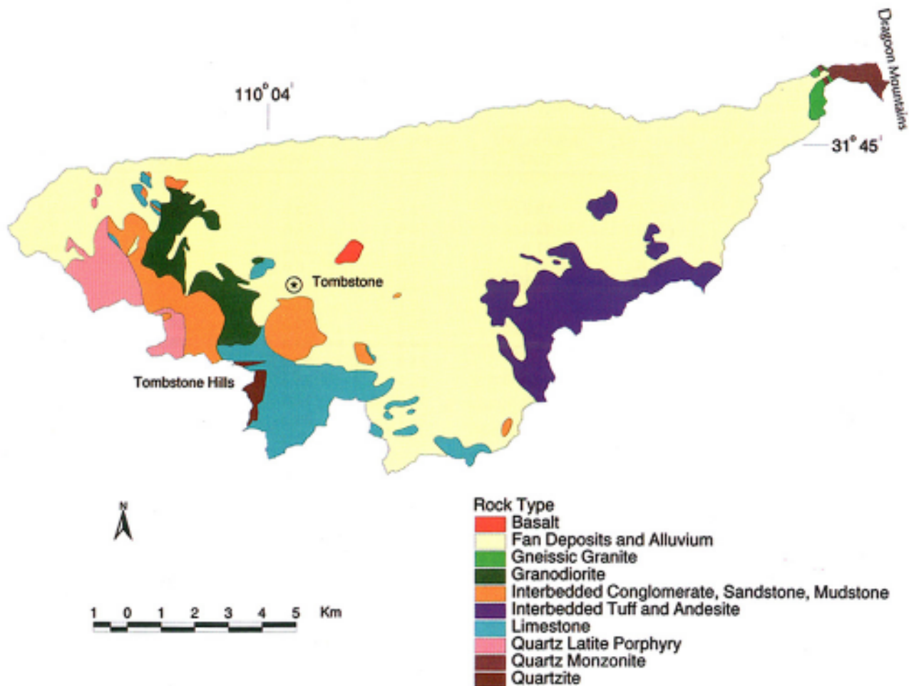
Figure 4 —Rock-type distributions in the Walnut Gulch Experimental Watershed (unpublished map, courtesy of S. N. Miller, ARS).
