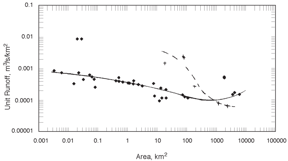
Figure 13 —Unit runoff as a function of drainage-basin area for Walnut Gulch and the San Pedro River (series 1), with additional data (+) and a relation line for the San Simon Wash Basin. Relation lines are visual interpretations of best fit.
