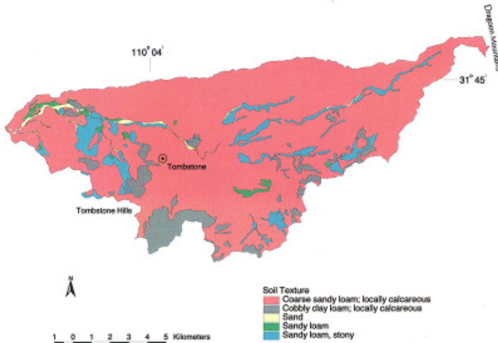
Figure 5 —Distributions of soil textures in the Walnut Gulch Experimental Watershed (unpublished map, courtesy of S. N. Miller, ARS).
