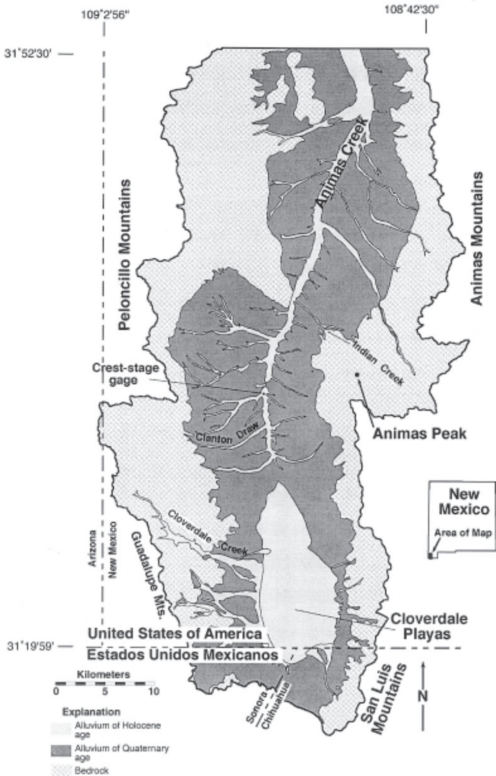
Figure 7 —Map of upper Animas Creek Basin, New Mexico and northern Mexico (Sonora and Chihuahua), showing the general geology. Areas of intermediate shading are bedrock, areas of dark shading are Quaternary alluvium, and areas of light shading along streams are Holocene alluvium (modified from Vincent and Krider 1998).
