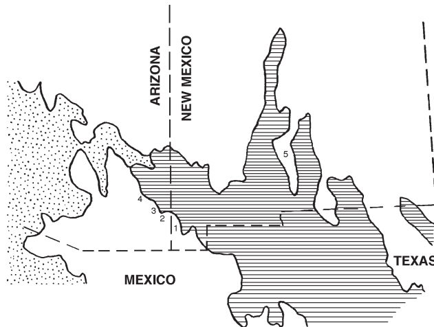
Figure 2 —Distribution of Sonoran Desert vegetation (stippled) and Chihuahuan Desert vegetation (stripped), separated by uplands and semiarid grasslands (no pattern), in southern Arizona, southern New Mexico, west Texas, and parts of northern Mexico (generalized from Shreve 1951, Schmidt 1979, and Brown and Lowe 1980). Locations of the Peloncillo, Chiricahua, Dos Cabezas, Graham, and San Andres Mountains are indicated by the numbers 1, 2, 3, 4, and 5, respectively.
