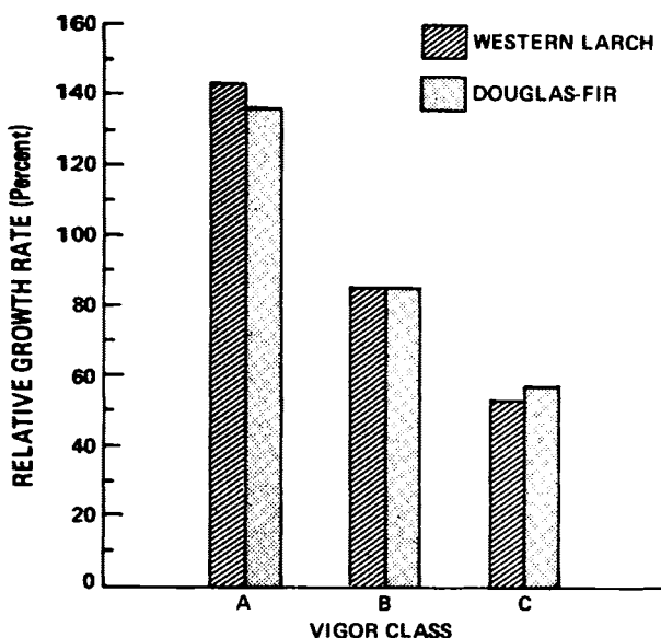
Figure 51. —Relationship of tree vigor to relative growth rates of western larch and Douglas-fir trees in cutover stands, western Montana. Relative growth rate = \frac{\text{Average growth rate for vigor class}}{\text{Average growth rate of all sample trees}} . These growth rates are based on board-foot increments of 416 western larch and 269 Douglas-fir trees. Relative growth rates of individual trees and of trees in uncut stands will differ from these.
