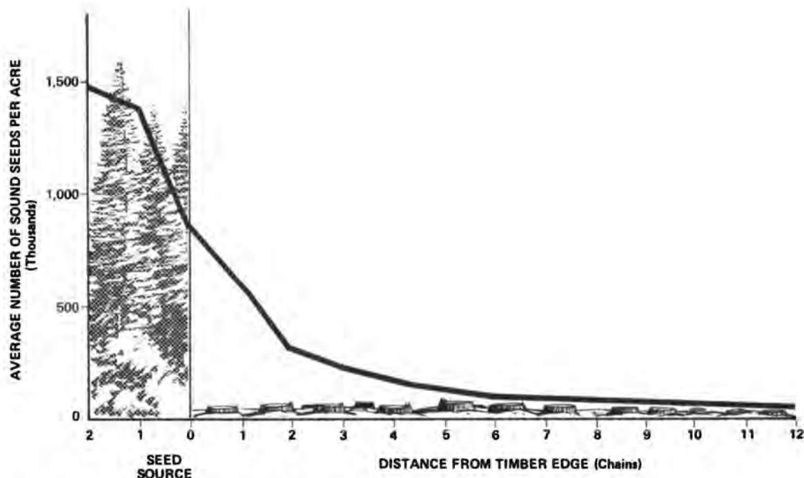
Figure 19.—Average number of sound western larch seeds dispersed per acre over three clearcut blocks from 1952 to 1957 by distance from seed source.
