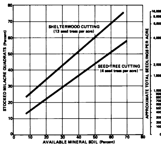
Figure 18.—Influence of cutting method and available mineral soil on establishment of first-year western larch seedlings.
