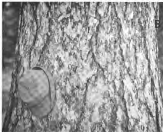
Figure 4.—Western larch bark structure is affected by age. Photo A shows the bark pattern of a 60-year-old fast-growing larch, while photo B shows the bark of a veteran that has grown over 600 years.
