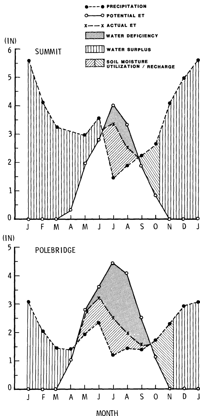
Figure 43.—Average water balance; schematic annual regime, based on the Thornthwaite method (see text) and 1951-80 monthly average temperature and precipitation.
