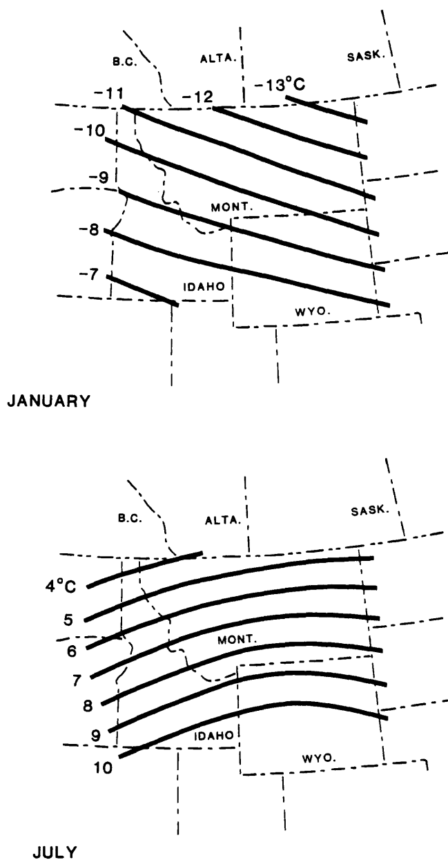
Figure 27.—Average temperature pattern ( ^{\circ}\text{C} ) in free atmosphere at 700-millibar pressure level (near 10,000 ft) over Northern Rockies, for January (A) and July (B). Based on 5 a.m., m.s.t., data for 13 years 1958-70; data were temperature values interpolated for 16 point locations from individual maps in monthly Climatological Data, National Summary.
