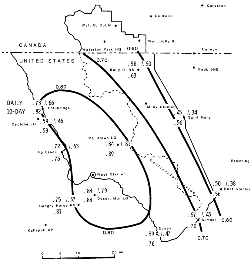
Figure 49.—Correlations of summertime precipitation, daily and 10-day, between West Glacier and other stations; based on available July and August 1946-72 data. Indicated daily coefficient ( r ) at left of slash is based on all days of record; value at right, on days with at least 0.01 inch at either station. Iso-lines are drawn for 10-day values of r .
