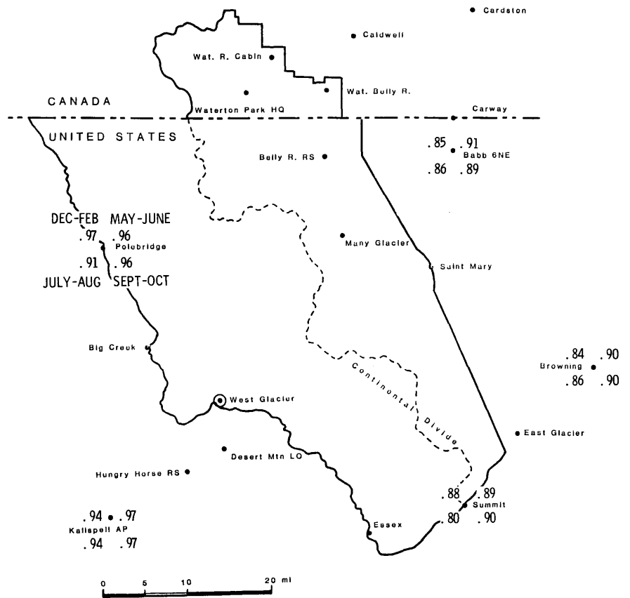
Figure 46.—Correlations of monthly average daily maximum temperatures, between West Glacier and other stations; based on 1949-80 data. Plotted numbers are averages of individual monthly correlation coefficients ( r ) grouped by indicated seasons.
