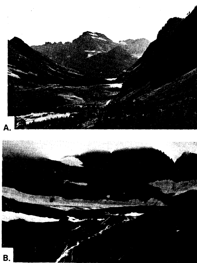
Figure 11.—(A) Broad setting of Grinnell Glacier (mostly hidden), toward distant right of center, and portion of Many Glacier area; viewed from northeast, in 1954. Hotel faintly visible on the near shore of Swiftcurrent Lake (middle distance, with Josephine Lake beyond). (B) Closer view of Grinnell Glacier (portion of ice surface visible) and the "Garden Wall," on cool, showery August 31, 1954.
