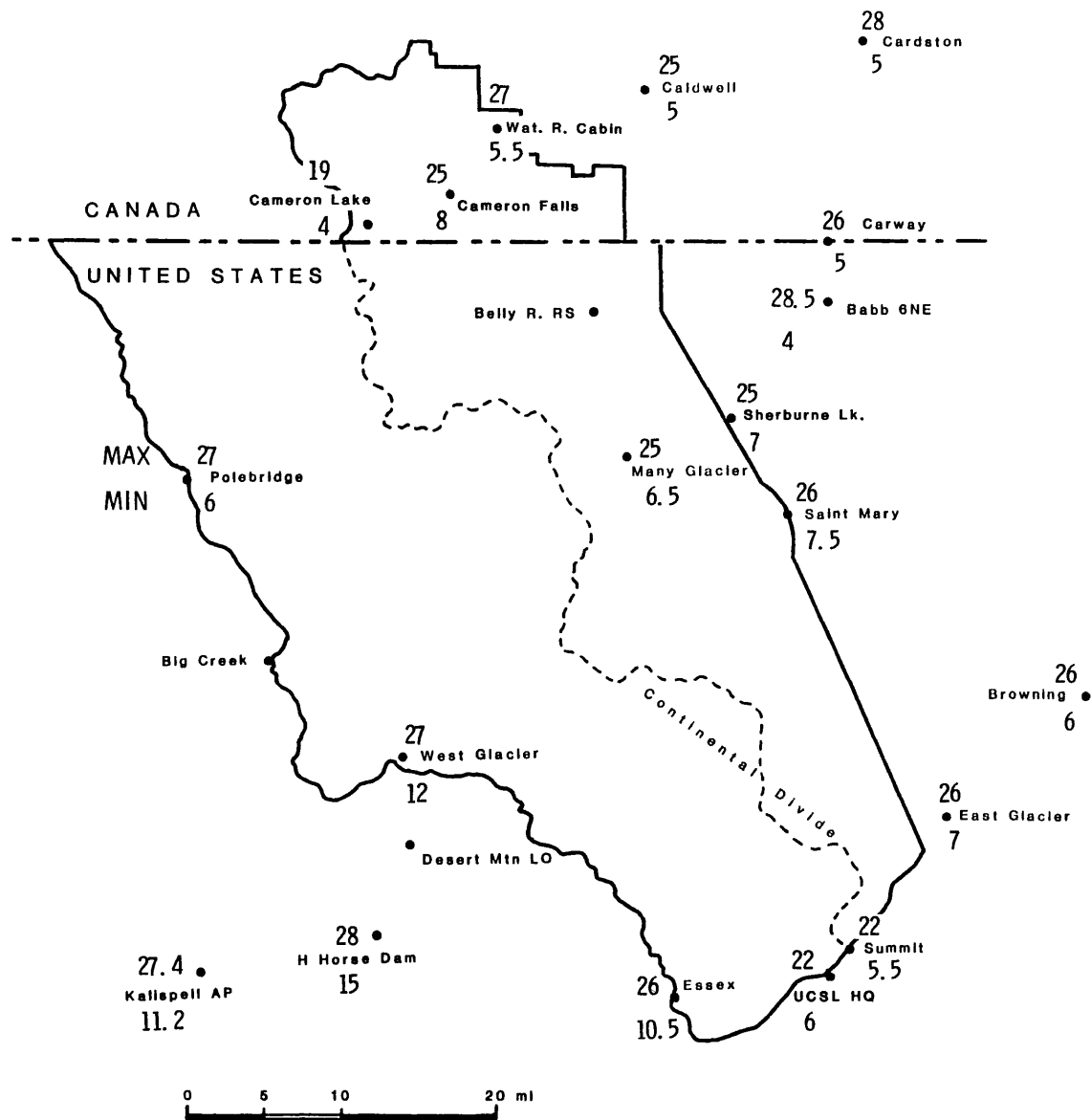
Figure 23.—Average daily maximum and minimum temperatures, °F, during January. Based on or adjusted to period 1951-80 and midnight-midnight observation day (the actual calendar day).
