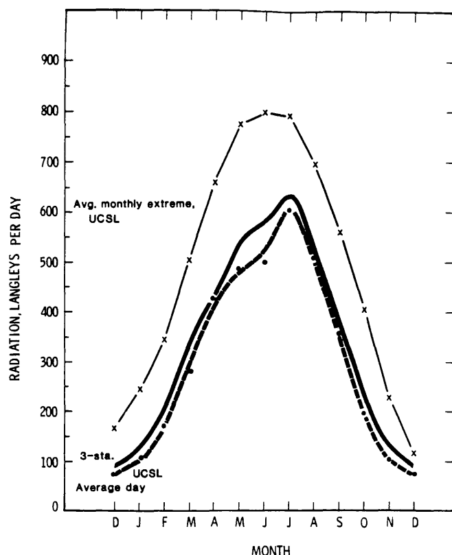
Figure 42.—Daily incoming solar radiation (direct and diffuse); annual regime. Langley's ( \text{gm-cal/cm}^2 ) received on a horizontal surface. Curves (and included data points) for Upper Columbia Snow Laboratory (UCSL) are based on 4-year period; three-station average based on 19 to 22 years at Great Falls, MT, Spokane, WA, and Suffield, AB.
