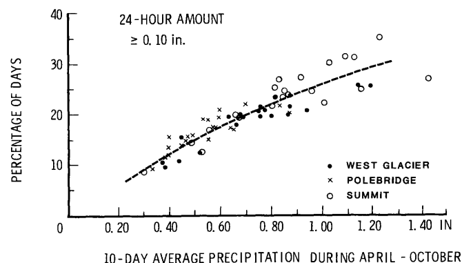
Figure 19. —Relationship between frequency of days with precipitation \geq 0.10 inch (2.5 mm) and the 10- (or 11-) day average precipitation, April-October. Based on 30 years 1949-78 at indicated stations. Dashed curve fitted by eye.
