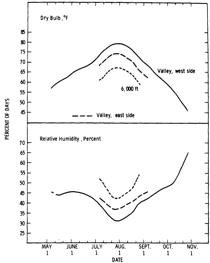
Figure 30.—Midafternoon dry bulb temperature and relative humidity; 10-day averages during fire season, smoothed by 1-4-1 weighting factor. Based on period 1951-80; mostly 1600 m.s.t. data (1300 beginning 1974). Curves for west-side valley are from combined record at Coram R.S. (1951-57) and Hungry Horse R.S. (1958-80); east-side valley, St. Mary R.S.; 6,000 ft, combined record at Desert Mountain (1951-73) and Firefighter Mountain (1975-80).
