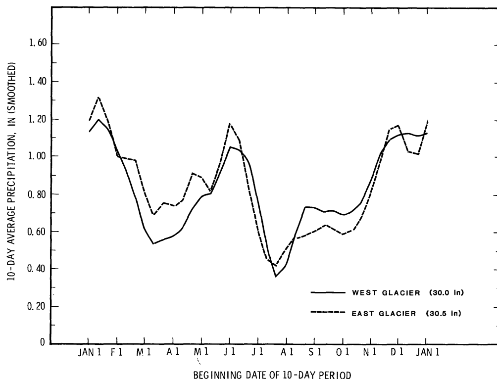
Figure 15.—Comparison of average annual precipitation regime at West Glacier and East Glacier, MT (annual totals shown in parentheses); based on 30 years of data, 1951-80. Lines connect plotted 10-day average values (or averages adjusted to 10-day period), smoothed by a running 1-2-1 weighting factor.
