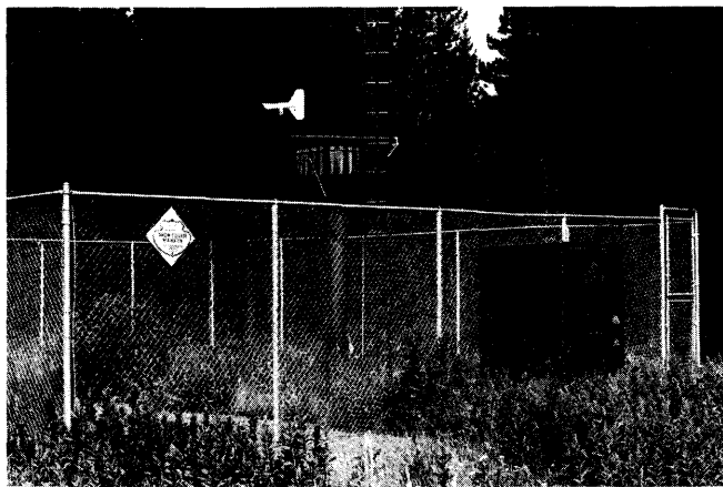
Figure 7.—SNOTEL (snow telemetry) station at Many Glacier; site between Ranger Station and Swiftcurrent Lake. Snow course is along fence; snow pillow, precipitation gauge with windshield, temperature sensor (inside vane-type shield), and antenna mast are within enclosure.
