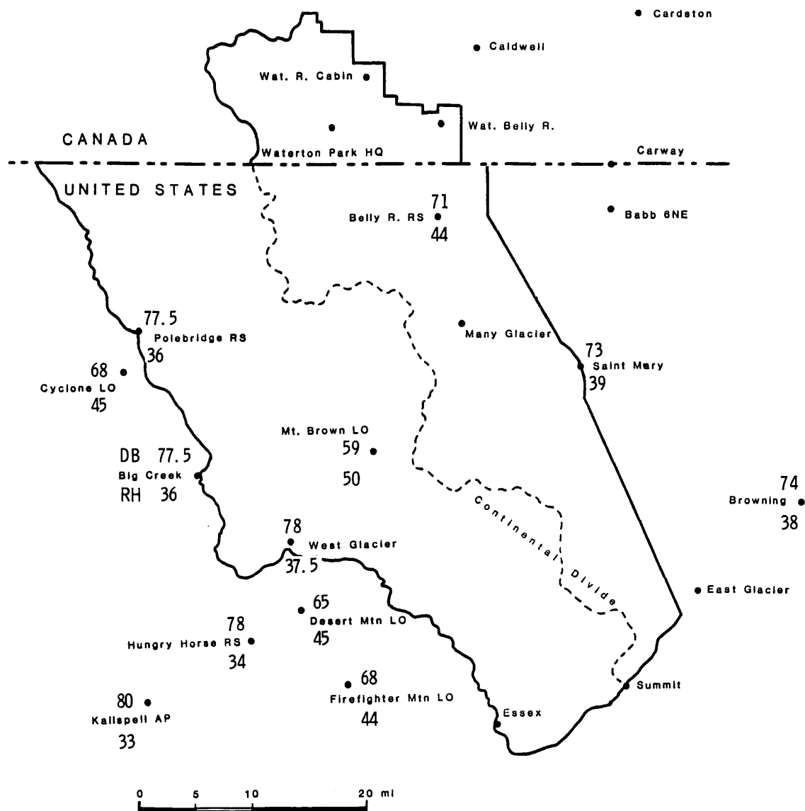
Figure 31.—Average midafternoon dry bulb temperature (DB), °F, and relative humidity (RH), percent, during July. Based on or adjusted to 1600 m.s.t. and period 1951-80.
