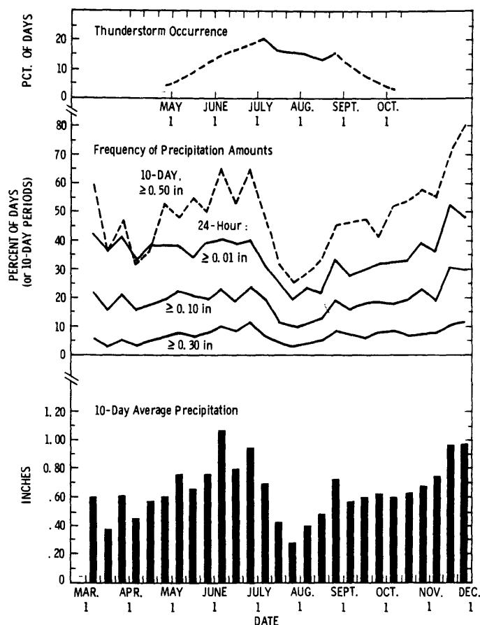
Figure 18. —Ten-day precipitation and thunderstorm occurrence, near west edge of Glacier Park; values plotted at middle of periods. Precipitation is two-station average from Polebridge and West Glacier, 1951-80. Amounts for 11-day periods are adjusted to 10 days. Thunderstorm graph for July and August is based on Desert Mountain Lookout, 1936-71 (storms within about a 20-mile radius); for other months (dashed line), occurrence is approximated from ranger station and Kalispell airport data.
