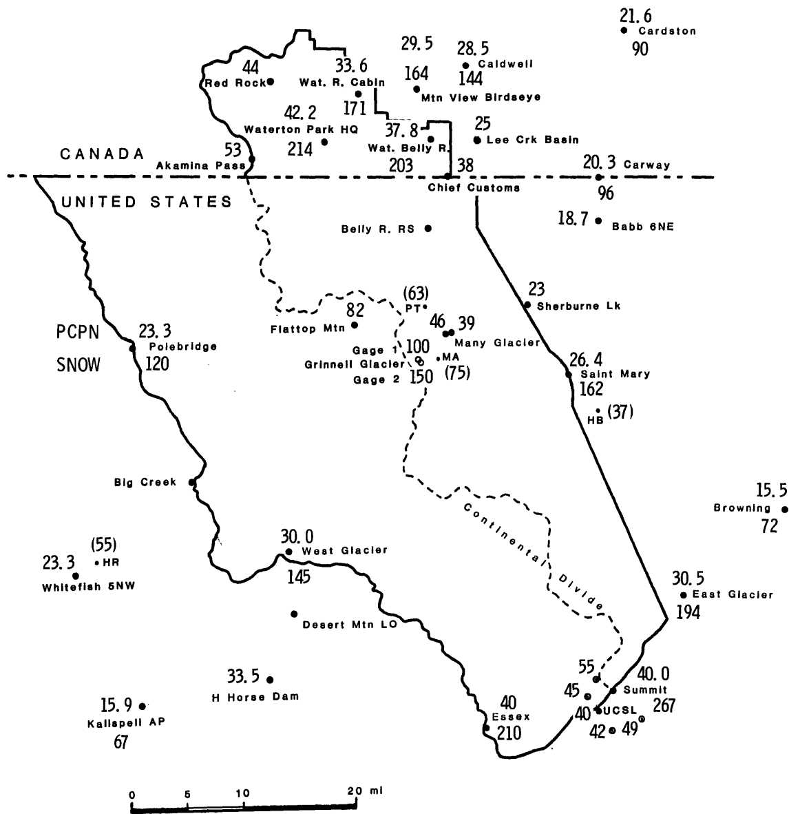
Figure 9.—Average annual precipitation (top or only number) and snowfall, inches, observed in and near Waterton-Glacier Park; based on or adjusted to normal period, 1951-80. Precipitation includes rain and melted snow (snowfall water content generally estimated at Canadian stations; see text). Number in parentheses is annual estimate based on snowpack data.
