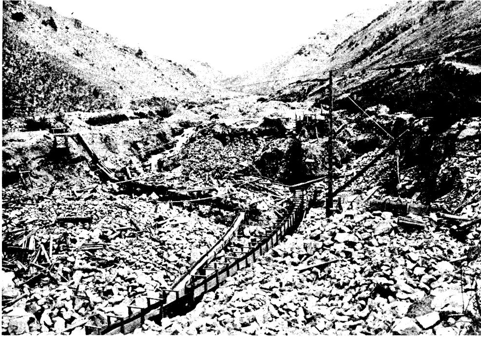
Figure 2a.—1871. An east-northeast view (elevation 6,000 ft) up Alder Gulch above Virginia City, MT. Placer mining following discovery of gold in 1863 caused extreme disturbance of canyon bottom. The south facing bluebunch wheatgrass covered slope at left supports a few mature Rocky Mountain juniper in rock outcrops. Juniper and Douglas-fir regeneration is evident. Conifers on north facing slope at right are Douglas-fir. Stumps in area indicate light cutting of trees. Wildfires had been relatively frequent in this locality. Examination of two fire-scarred stumps showed evidence of four fires before 1871. Photograph by W. H. Jackson, courtesy of Montana Historical Society.
