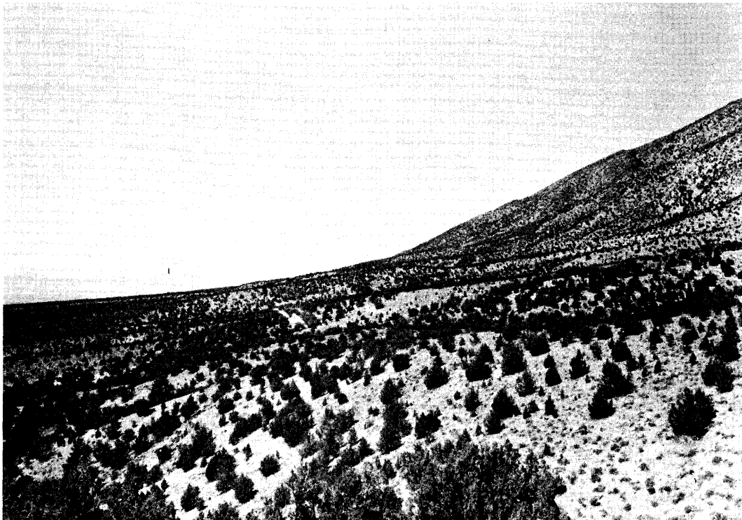
Figure 5b.—September 3, 1976. Juniper has increased in all areas, and young trees and seedlings are abundant. The increase has been greatest in the areas of low slope angle and least on the mountain slopes at right. Photograph by Gary Rogers, photograph courtesy of Gary Rogers and the University of Utah Press.
