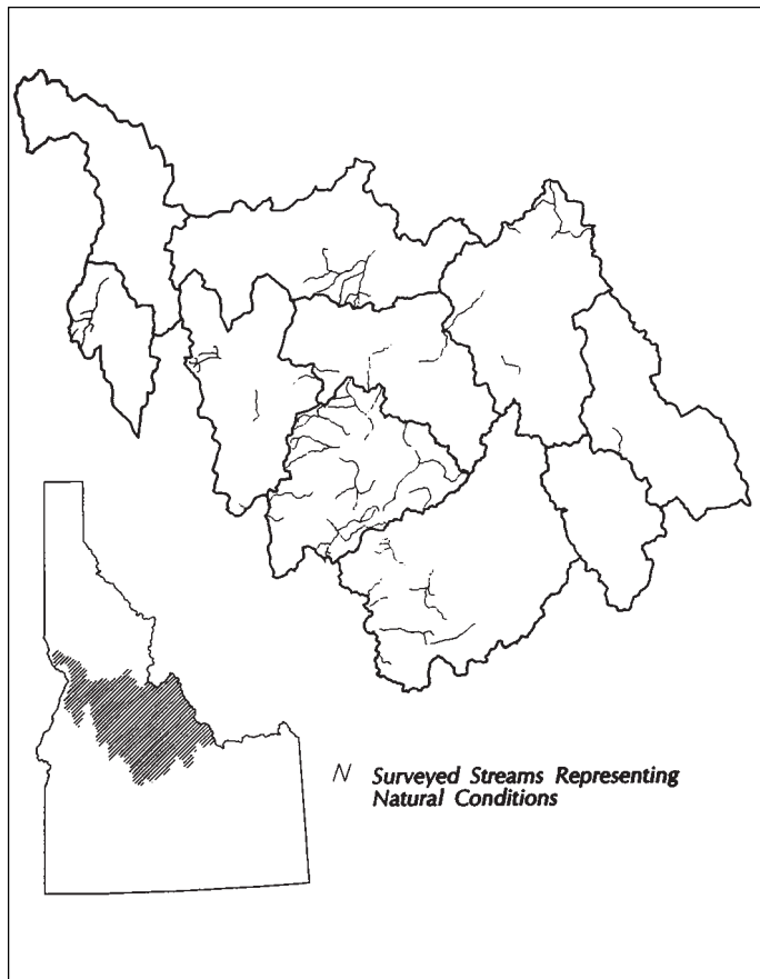
Figure 1 —General location of streams that were surveyed to develop the "natural condition" data base.
