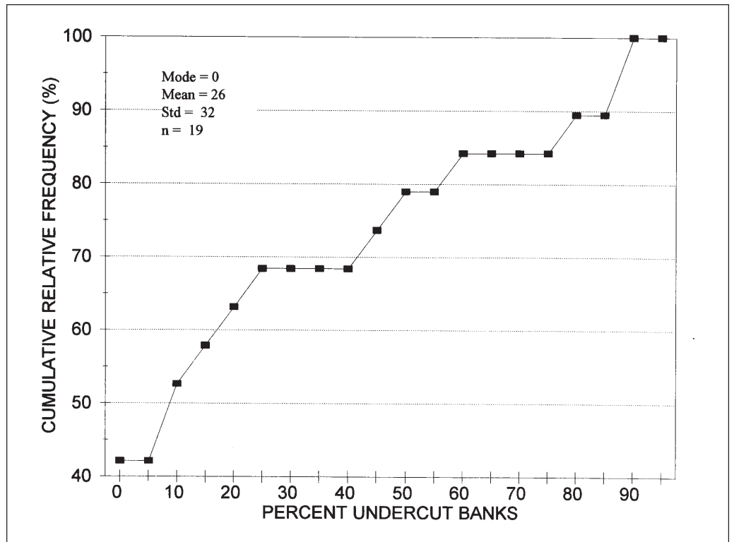
Figure 47 —Cumulative relative frequency distribution displaying the range of percent bank undercut for “C” channel sedimentary stream reaches.
