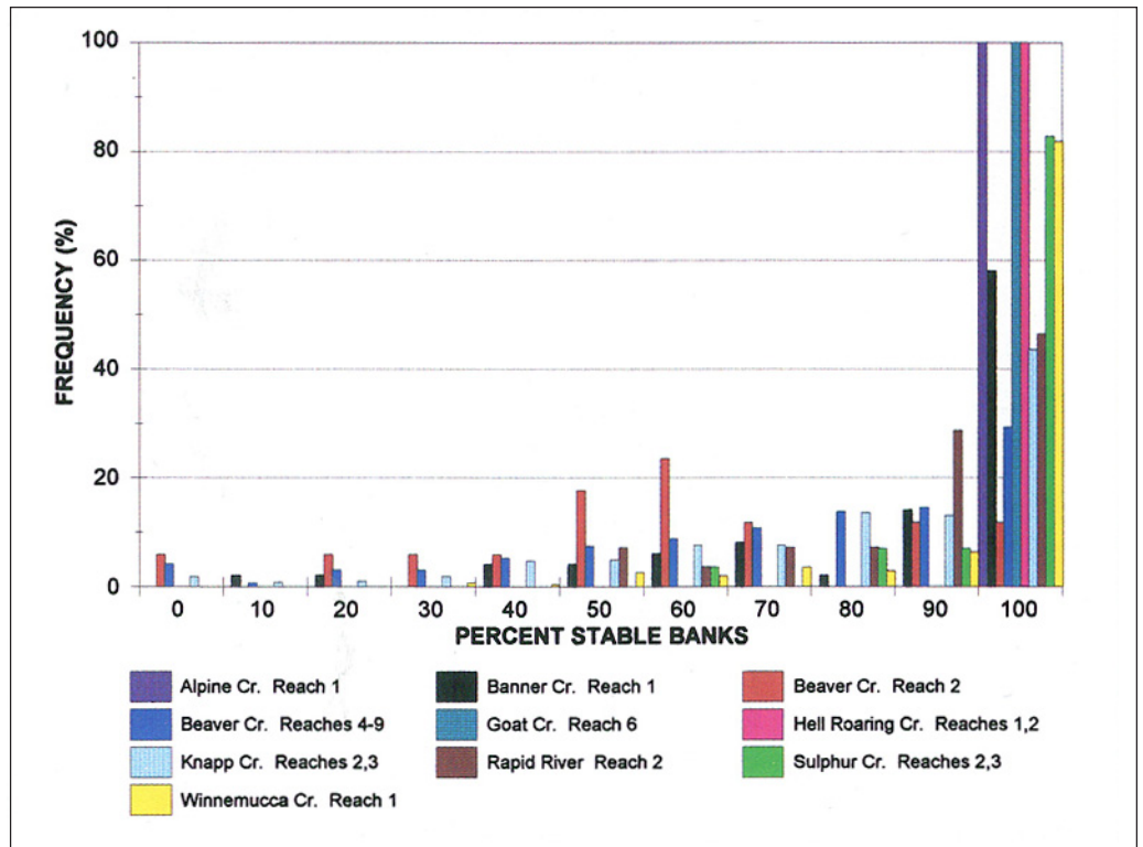
Figure 6 —Frequency distribution displaying the range of percent bank stability or “C”-wooded granitic stream reaches.
