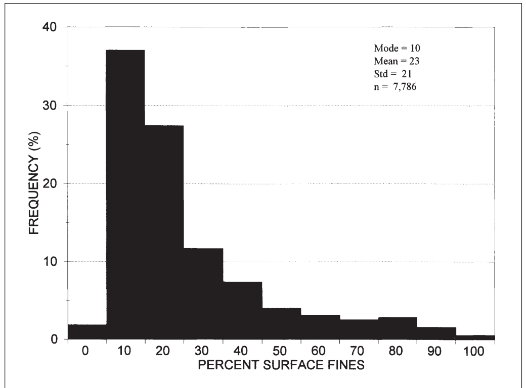
Figure 132 —Frequency distribution displaying the range of percent surface fines for “B” channel reach types.
