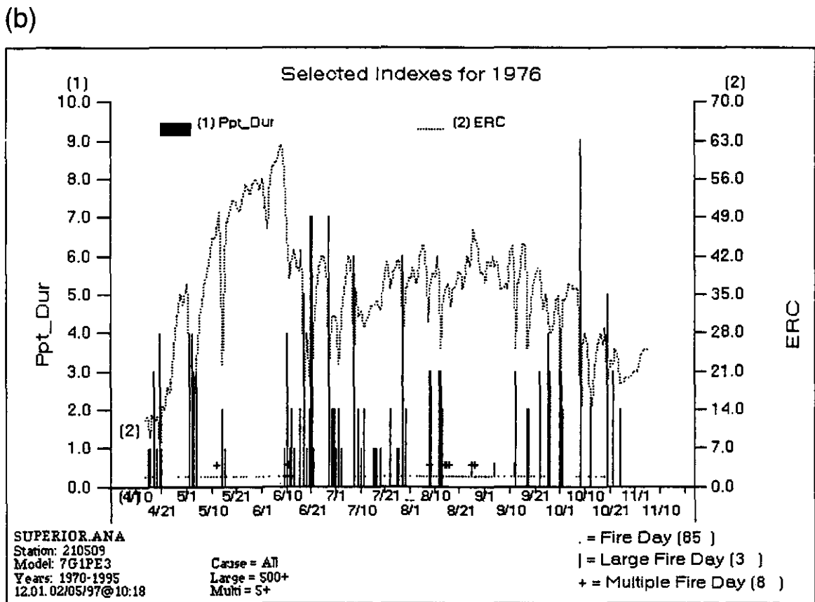
Figure 10 —Selected indexes. Superior National Forest. (a) Keetch Byram Drought Index (KBDI) and precipitation amount for 1976, (b) Energy Release Component and precipitation duration for 1976.
