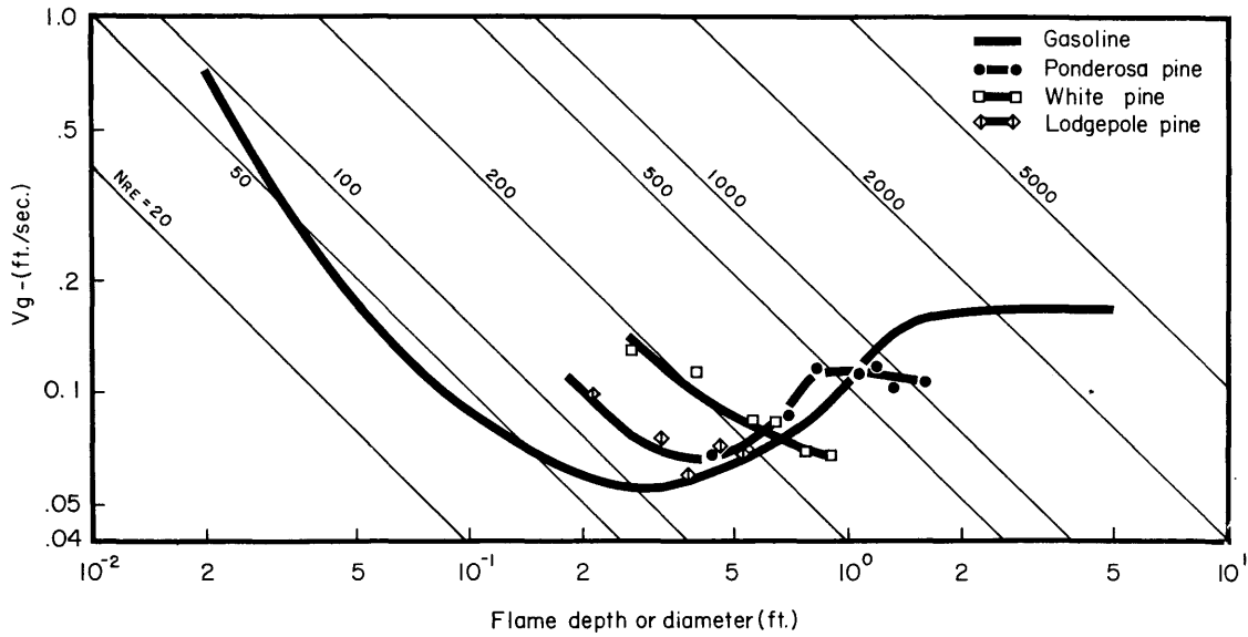
Figure 6.--Burning regimes of various fuels based on cold vapor density and viscosity.
