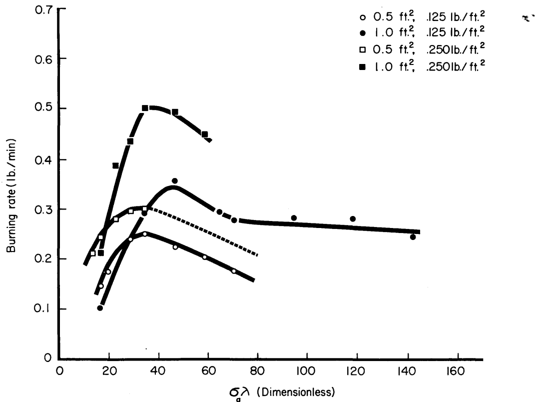
Figure 9.--Influence of porosity, \lambda , on burning rate for fires in ponderosa pine needles with a \sigma_a of 1,740 ft. 2 /ft. 3 . Each data point is average of three fires.
