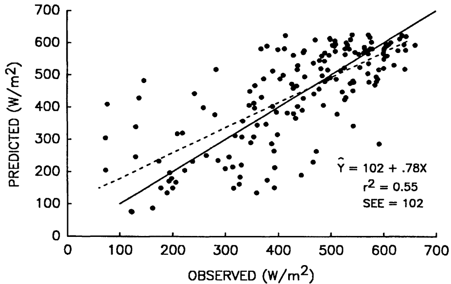
Figure 3 —Regression of incoming solar radiation predicted by MTCLIM vs. actual radiation observed at Ambrose S. Broken line is the regression line and the solid line is the 1:1 line (intercept = 0; slope = 1.0).
