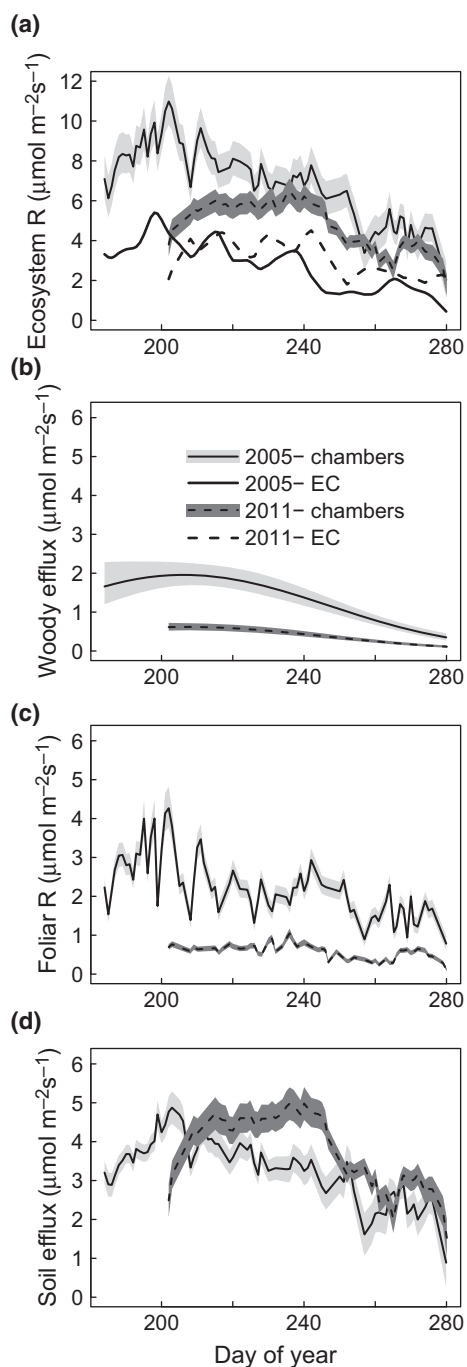
Fig. 4 R_e estimated by EC and chambers for 2005 ( 65 \text{ m}^2 \text{ ha}^{-1} healthy tree basal area), and in 2011 ( 10 \text{ m}^2 \text{ ha}^{-1} healthy tree basal area). (a) EC estimates of R_e are significantly lower than chamber estimates, and EC R_e did not decline over 2005–2011 period, while chamber estimates of R_e decreased 35%. The shaded area is 95% confidence interval (CI), and EC values are smoothed splines of nightly mean NEE measurements where u^* > 0.2 \text{ m s}^{-1} . Modeled respiration and 95% CI from chambers in 2005 and 2011 for woody tissues (b), foliage (c), and soils (d). Respiration declined 72% for live wood 74% for foliage, but soil respiration was greater in 2011.
