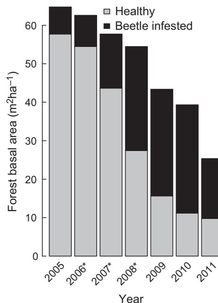
Fig. 2 From 2008 to 2011, the bark beetle epidemic greatly reduced live basal area at GLEES. In 2011, only 15% ( 10 of 65 \text{ m}^2 \text{ ha}^{-1} ) of the original forest basal area remained alive and uninfested by bark beetles. Mortality survey was not conducted 2006–2008 (marked *), numbers are estimated from dendrological data (see text for details).
