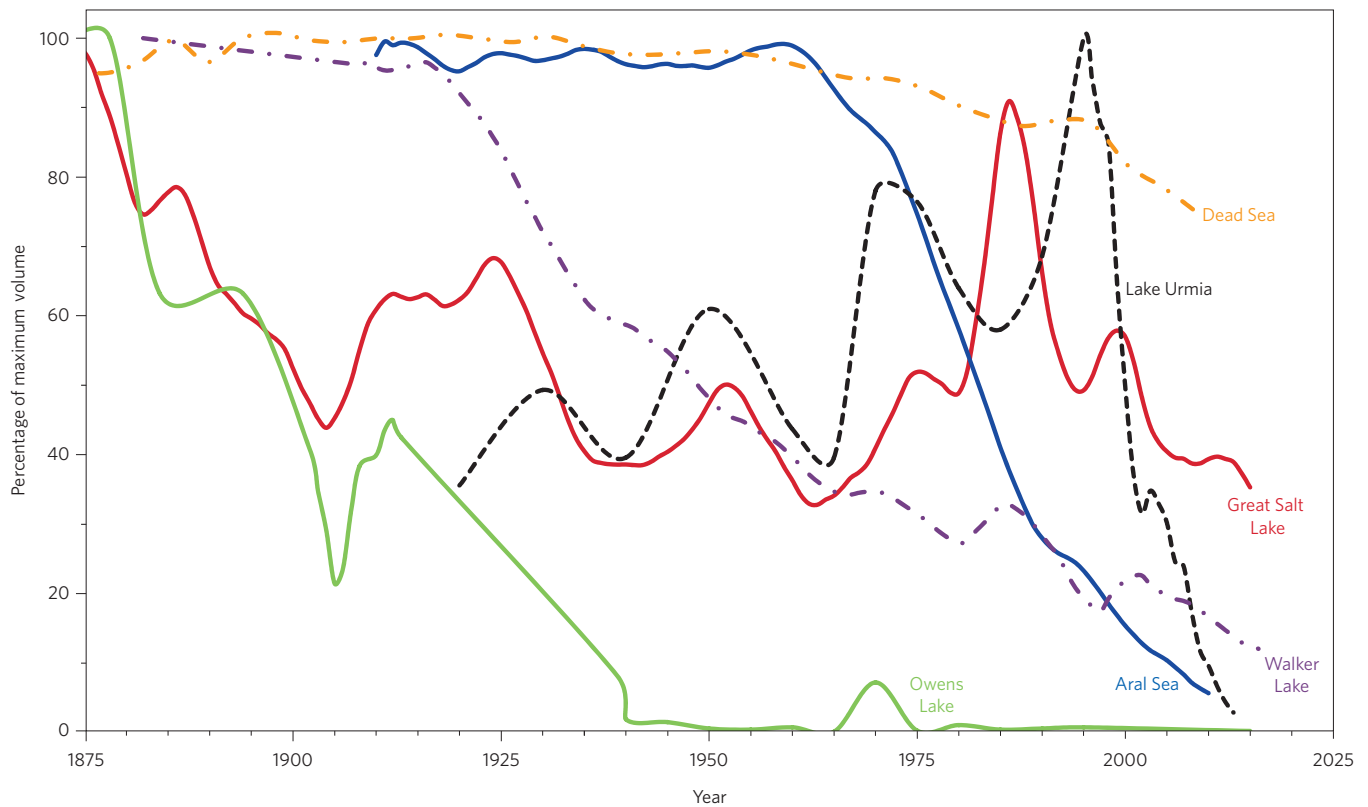
Figure 2 | Major decreases in the water volumes of important saline lakes over the past 140 years (five-year running averages). Note that the relatively small fractional decline in the volume of the Dead Sea can be explained by its great depth; the elevation of the Dead Sea has been reduced by over 28 m during this time period and impacts have been pervasive 43 . Recently, Lake Urmia has declined most precipitously from a combination of agricultural water development and drought. See Methods for details.
