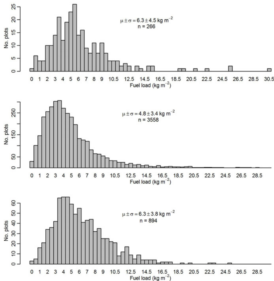
Figure 4. The distribution of surface fuel loading for the FIA plots of three FTGs: loblolly/shortleaf pine (160), Douglas fir (200), and California mixed conifer (370).
