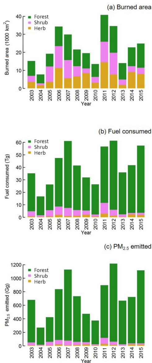
Figure 10. Annual burned area, fuel consumed, and PM 2.5 emitted for 2003–2015.
