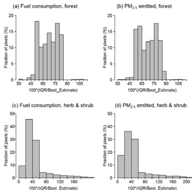
Figure 20. Distribution of relative interquartile range from pixel-level Monte Carlo style simulations.
