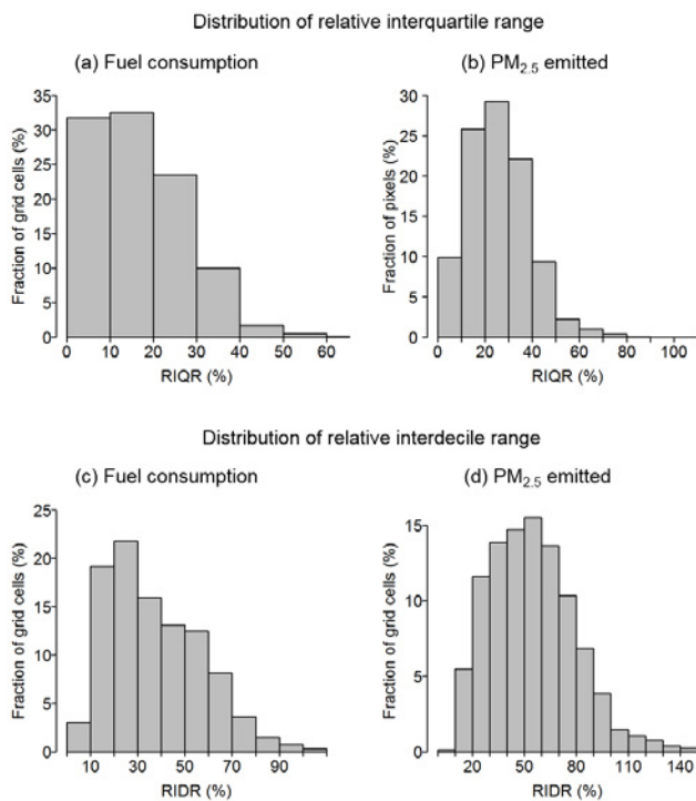
Figure 21. Distribution of relative interquartile range (a, b) and relative interdecile range (c, d) from 10 km × 10 km gridded Monte Carlo simulations.
