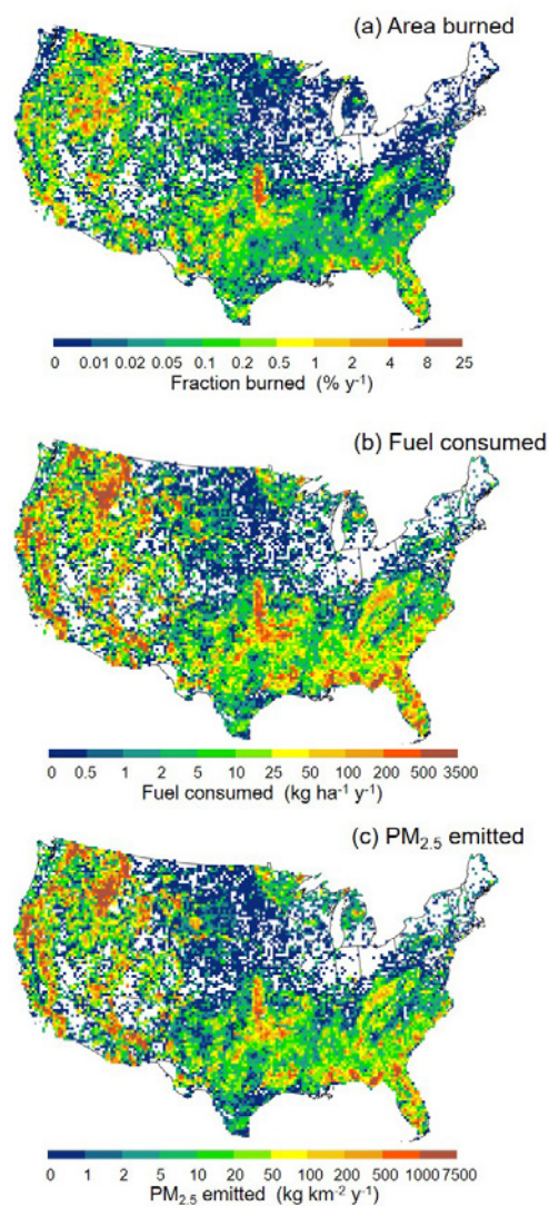
Figure 11. Annual burned area, fuel consumed, and PM 2.5 emitted averaged over 2003–2015.
