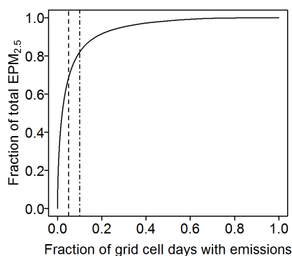
Figure 17. Cumulative distribution of daily PM 2.5 emissions aggregated on a 10 km × 10 km grid. The dashed line and dashed–dotted line mark 5 % and 10 % of grid cell days with emissions.
