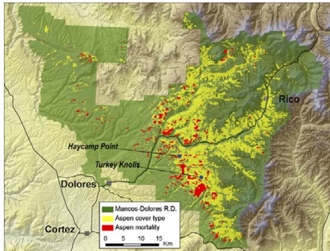
Fig. 3. Concentrated patches of recent aspen mortality detected by aerial sketch-mapping, distribution of aspen cover type, and locations of stand sampling on the Mancos-Dolores Ranger District, San Juan National Forest.
