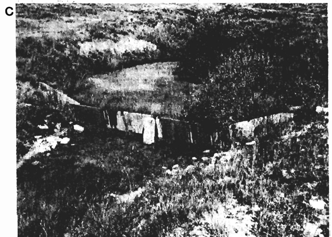
Figure 5.—The appearance of the site occupied by a larger gully control structure at the mouth of Alkali Creek in western Colorado: (a) immediately after treatment in 1963, (b) in 1964, and (c) 12 years later in 1975.
