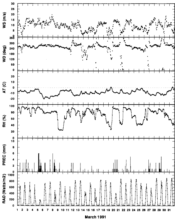
Figure 7.2.—Meteorological time plot, Glacier Lakes, March 1991; same abbreviations as in figure 7.1.
