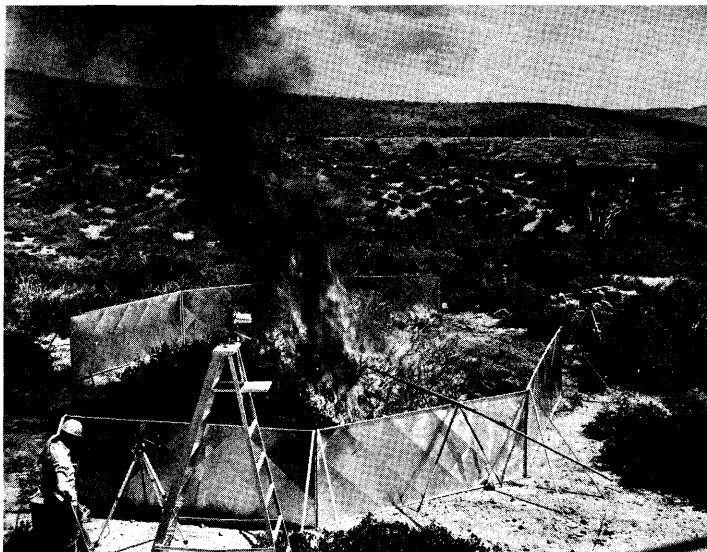
Figure 3.--A typical research fire and area fuel distribution in oak chaparral on the Prescribed Fire Experimental Area, near Prescott, Arizona. Note the heat sink-thermocouple-radiation sensing package in the center of the burning line (feedout underground), heat flux transducer (horse), 35-mm camera and "midflame height" anemometer (right center), 16-mm time-lapse camera (on ladder), infrascopes (on tripod), and power sprayer (to extinguish sample area at end of flaming combustion; lower left corner). Not shown are 36-foot tower (from which photo was taken) with another 16-mm time-lapse camera, and a 20-foot standard anemometer.
