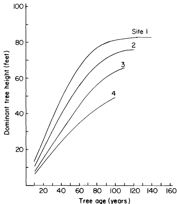
Figure 2.—Site quality curves for Colorado aspen based on Baker's (1925) site quality criteria.
