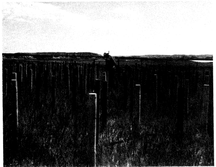
Figure 2.-The poorly drained plot near Scenic has a clay soil with pH of 8.2. Note that soil has washed into the plot from the surrounding area.
