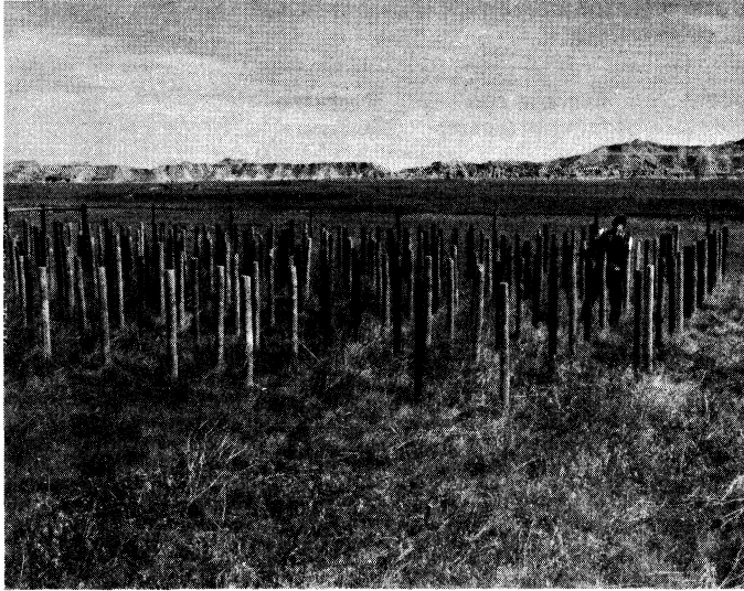
Figure 3.-The well-drained plot near Scenic has a clay soil with pH of 7.4. This plot has no washed-in soil. Posts are being tested with the 50-lb lateral pull.
