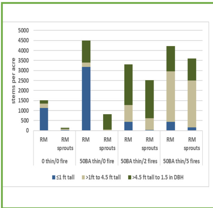
Figure 1 —From four treatments on the Bankhead National Forest, Alabama, red maple reproduction by all tallies and tallies that are sprouts.
