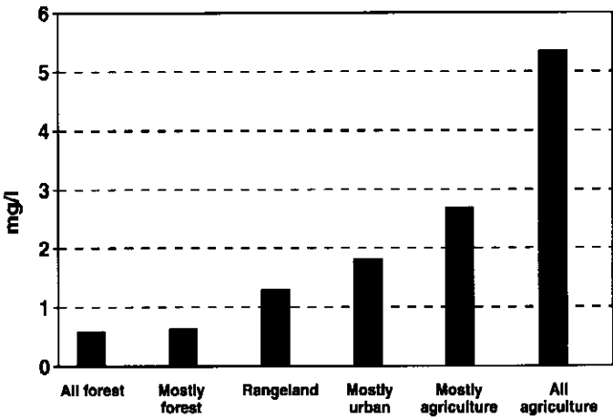
Figure 3.—Nitrogen concentration by land cover (from Omernik 1977)
