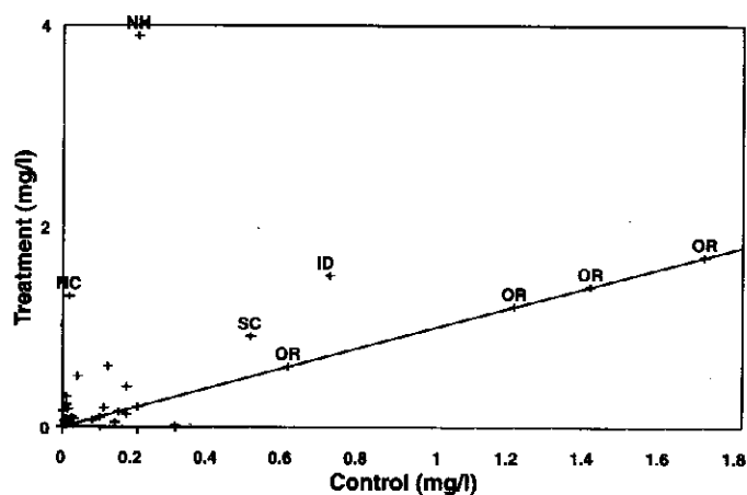
Figure 5.—Response of streamwater nitrate-N concentrations to forest harvesting at experimental watersheds (see table 4 for details) (state abbreviations identify watersheds with largest concentrations)
