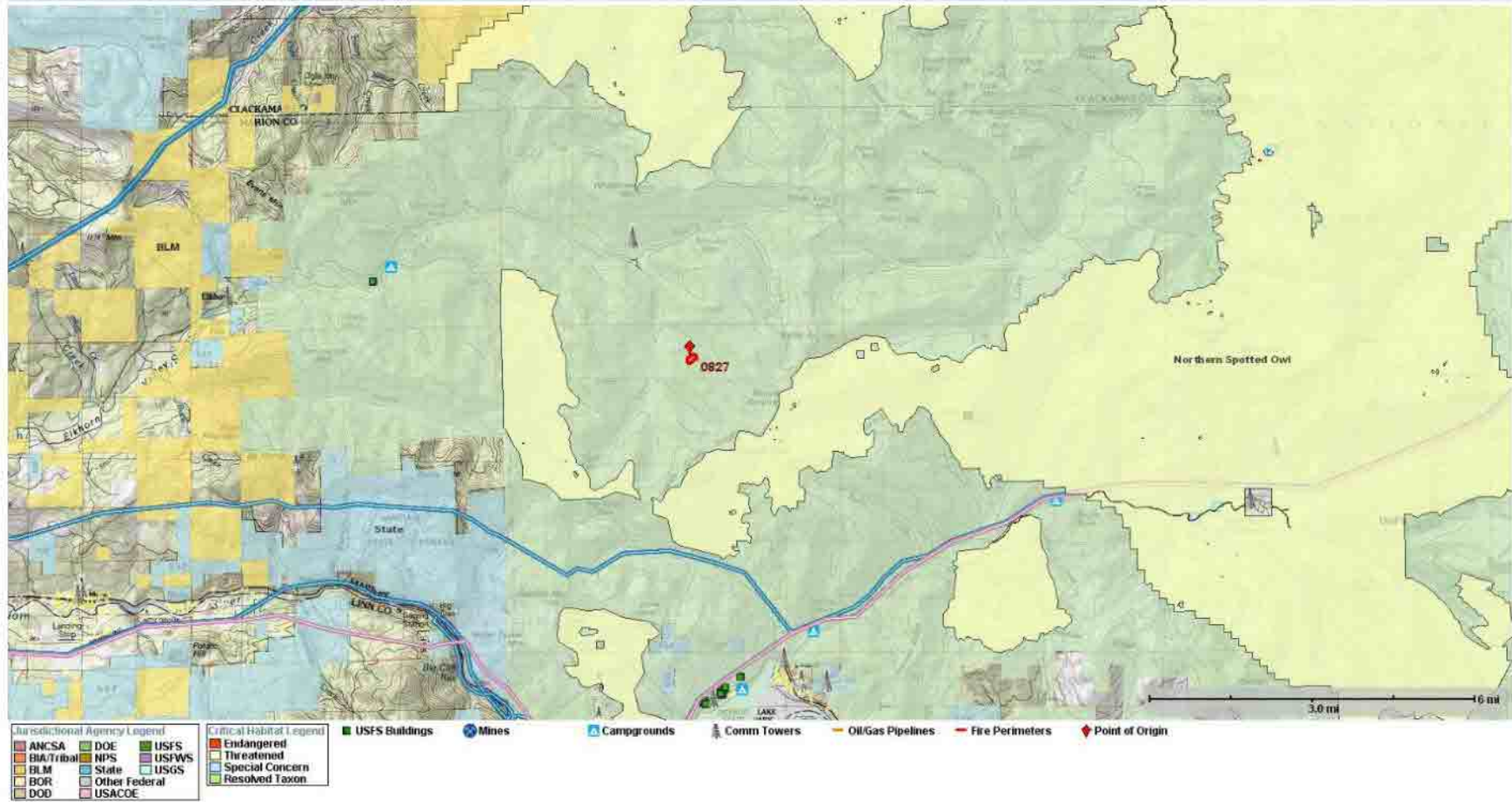
Beachie Creek HVRAs
