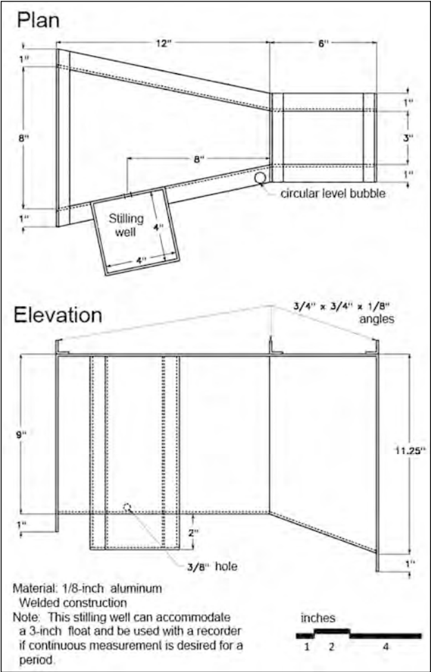
Figure 10.2.—Working drawing of modified 3-inch Parshall flume.
