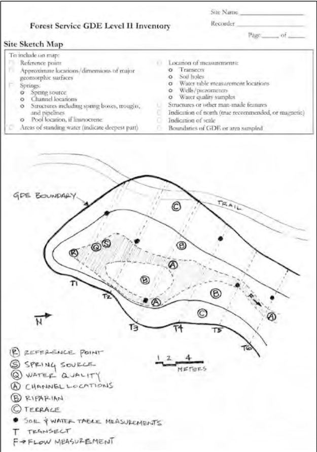
Figure 4.—Site sketch map example.
