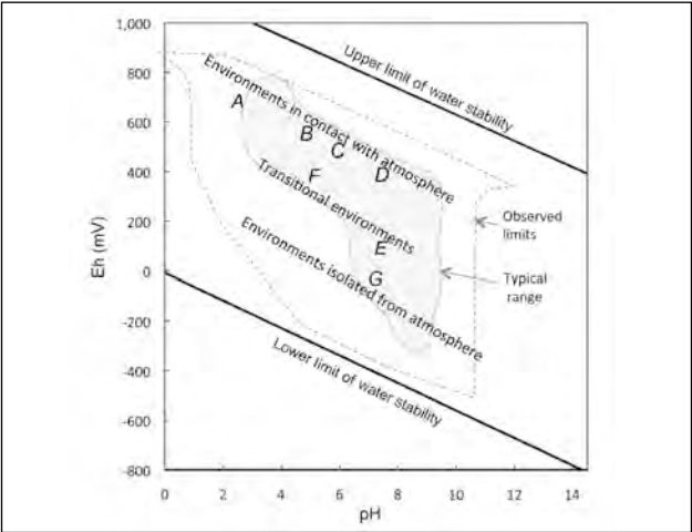
Figure 6.—Distribution of Eh-pH values in natural aqueous environments. Zone A is acidic mine drainage, B is rain, C is stream water, D is ocean water, E is groundwater, F is bog water, G is anaerobic wetlands (redrawn from Langmuir 1996 and Baas-Becking et al. 1960).
