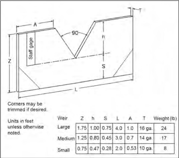
Figure 10.1.—Portable weir plate sizes.
