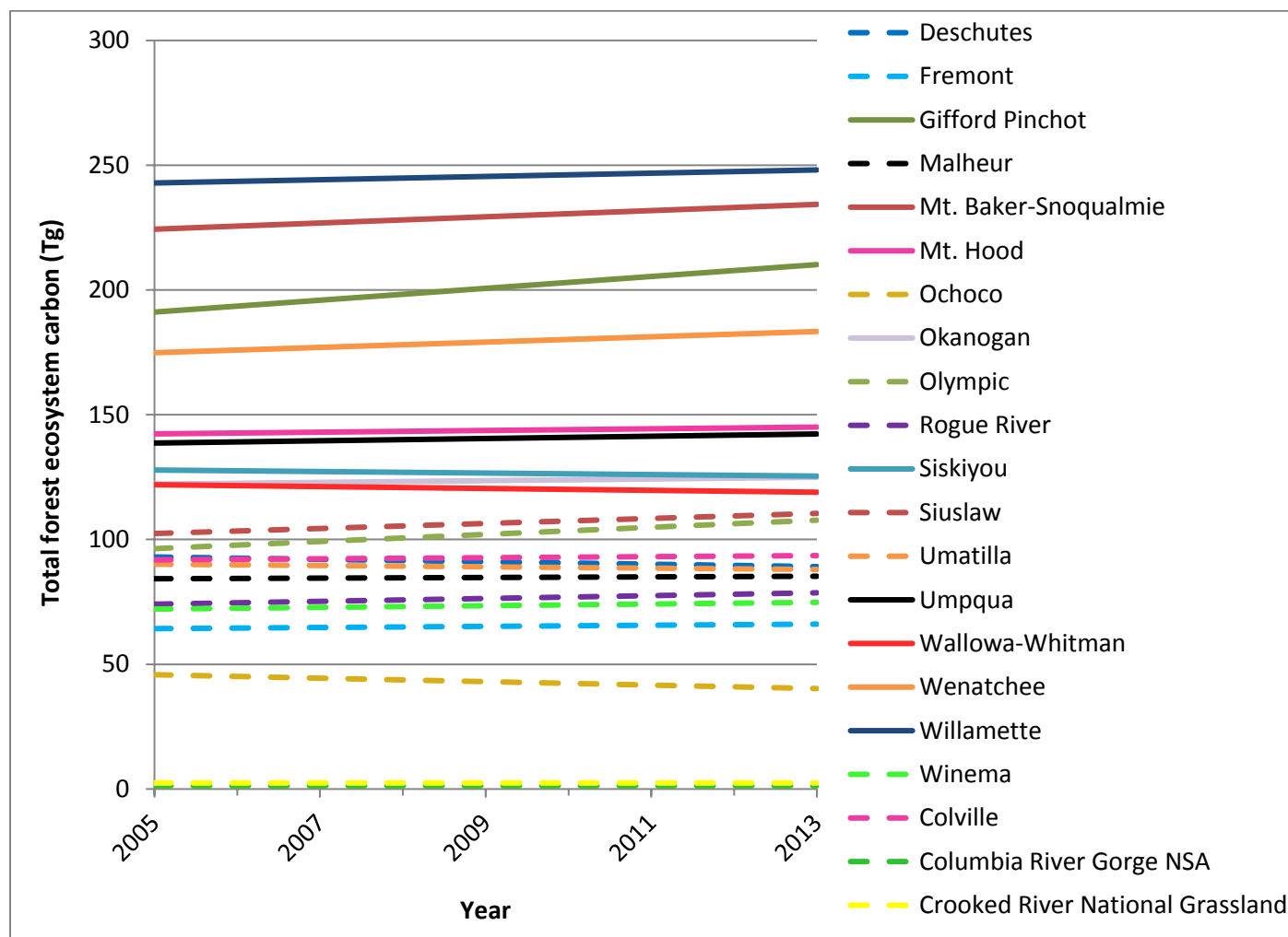
Figure 4. Total forest ecosystem carbon (Tg) for the national forests and grassland in the Pacific Northwest Region from 2005 to 2013.
