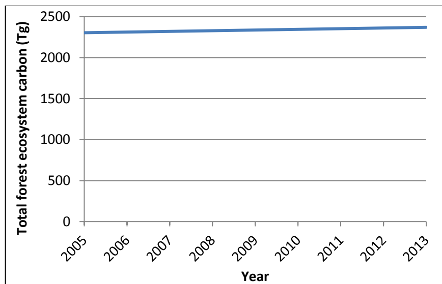
Figure 3. Total forest ecosystem carbon (Tg) for the Pacific Northwest Region from 2005 to 2013.
