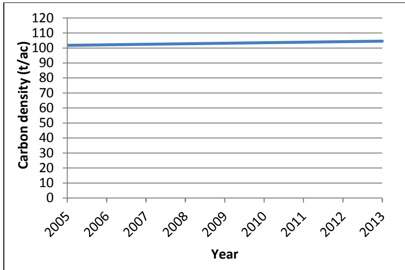
Figure 6. Carbon density (tonnes/acre) for the Pacific Northwest Region from 2005 to 2013.
