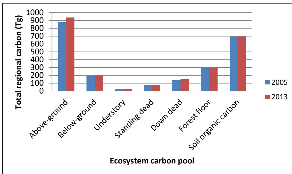
Figure 5. Carbon stocks in the seven forest ecosystem pools in national forest lands of the Pacific Northwest Region for 2005 and 2013.
