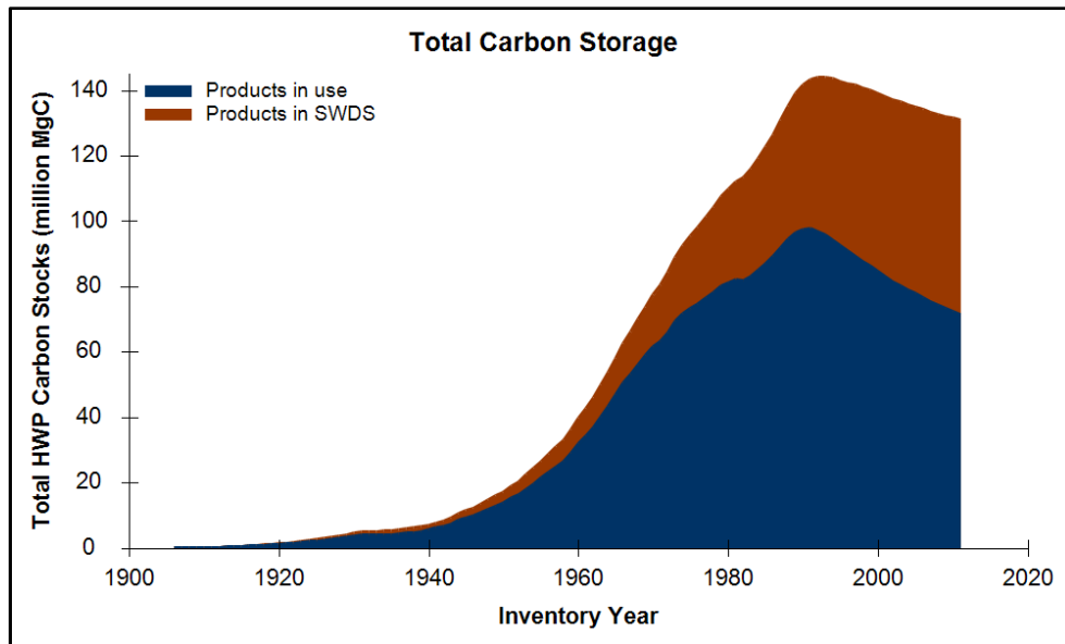
Figure 9. Cumulative total carbon stored in HWP manufactured from Pacific Northwest Region timber using the IPCC/EPA approach. Carbon in HWP includes both products that are still in use and carbon stored at solid waste disposals sites (SWDS), including landfills and dumps (Butler et al. 2014).
