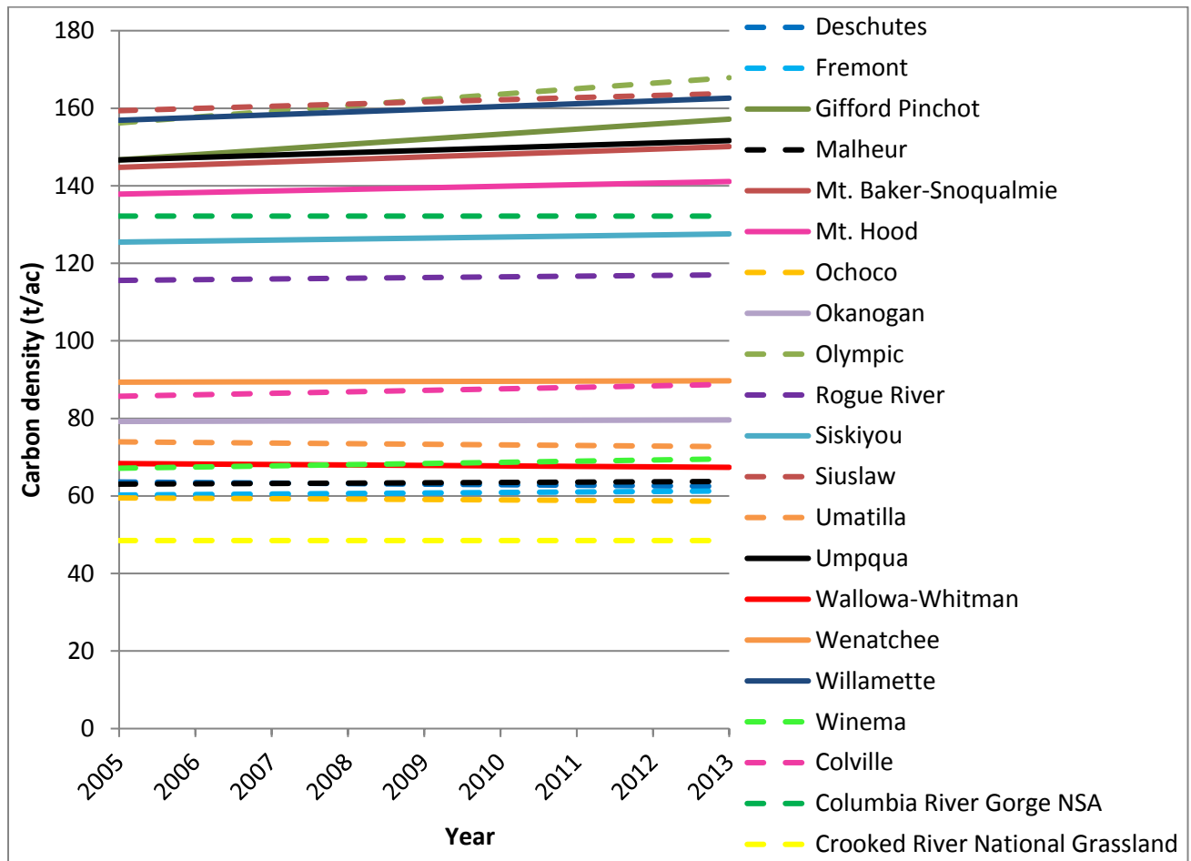
Figure 7. Carbon density (tonnes/acre) for the national forests and grassland in the Pacific Northwest Region from 2005 to 2013.
