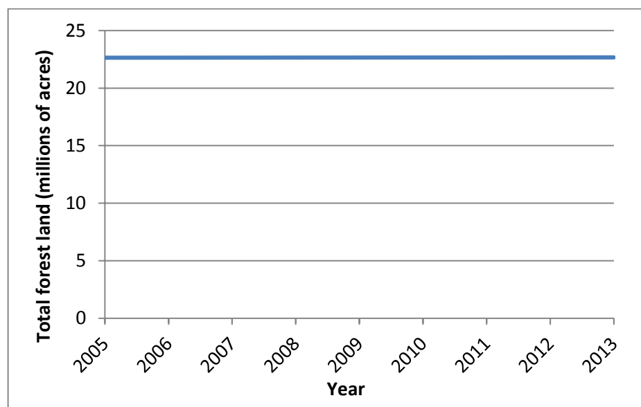
Figure 2. Total forest land (millions of acres) in national forests in the Pacific Northwest Region from 2005 to 2013.
