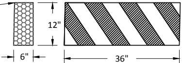
BARRICADE, BM-L-36, BM-R-36 RED ON WHITE A 3" X 36" HORIZONTAL STRIP OF SILVER REFLECTIVE SHEETING SHALL BE FASTENED TO THE BACK OF THESE BARRICADE MARKERS.
