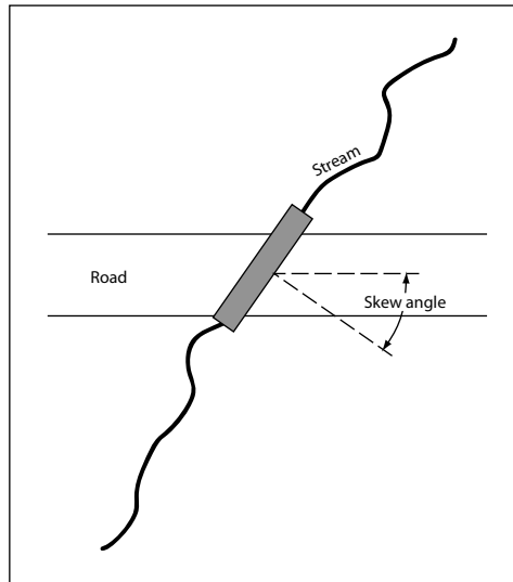
Figure E-7. Measurement of culvert skew.
