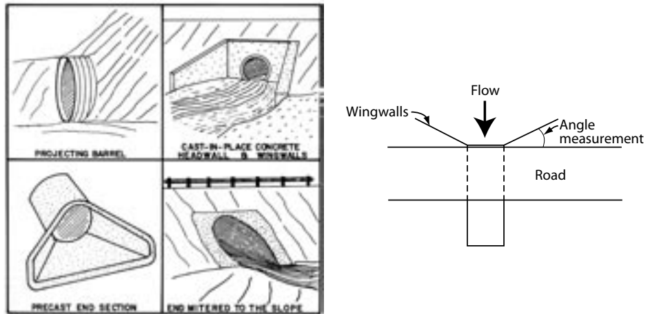
Figure E-6. (from Normann et al 2001). Inlet type examples (clockwise from top left): projecting, headwall and wingwall, mitered and metal or cement end section. Wing-wall measurement is illustrated here.
