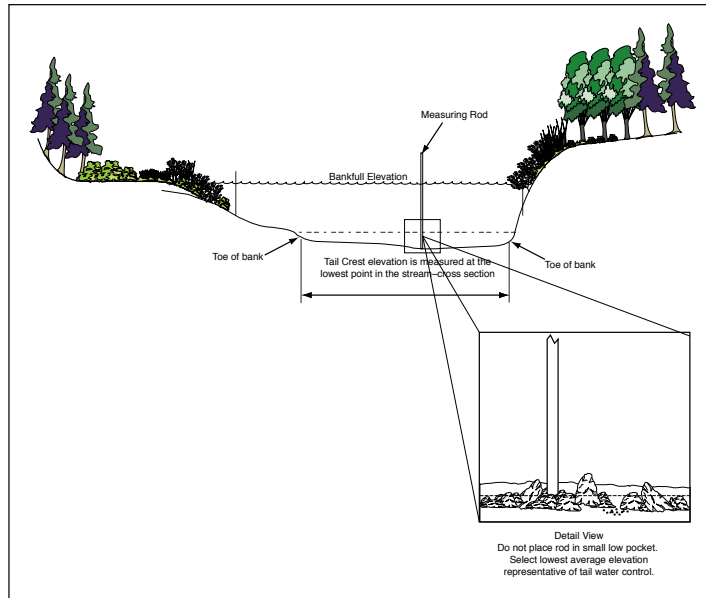
Figure E-14. Measuring the tailwater control.
