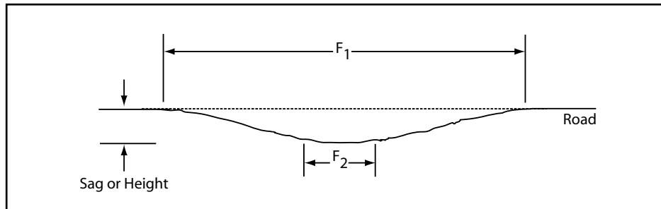
Figure E-3. Low water ford (unvented)
