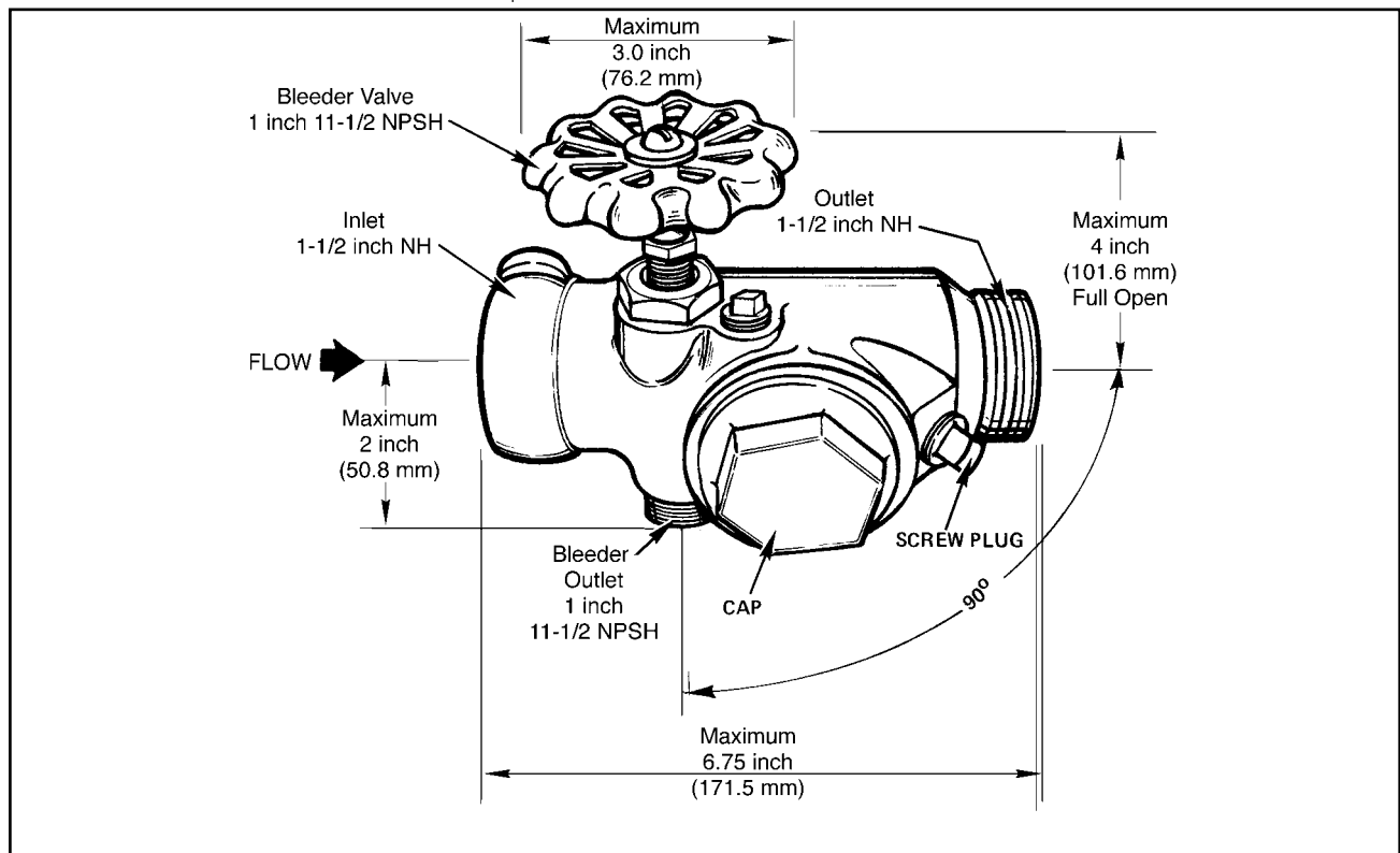
Figure 1. Check and bleeder valve configuration.
