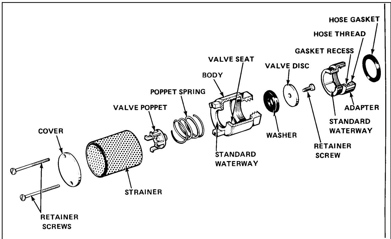
Figure 1. Foot valve and strainer configuration.
