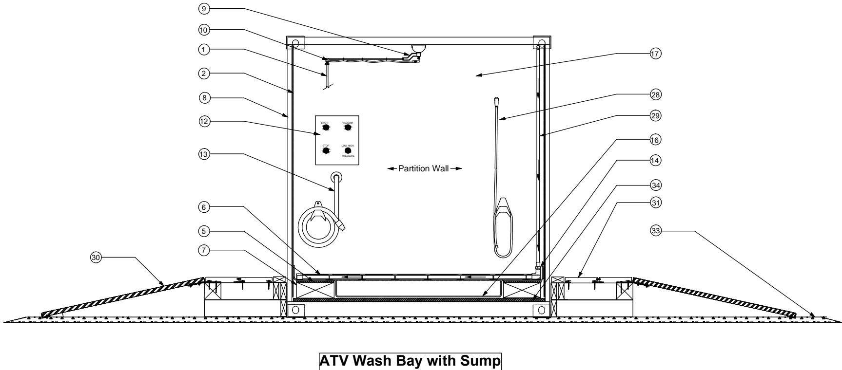
Section B 4
