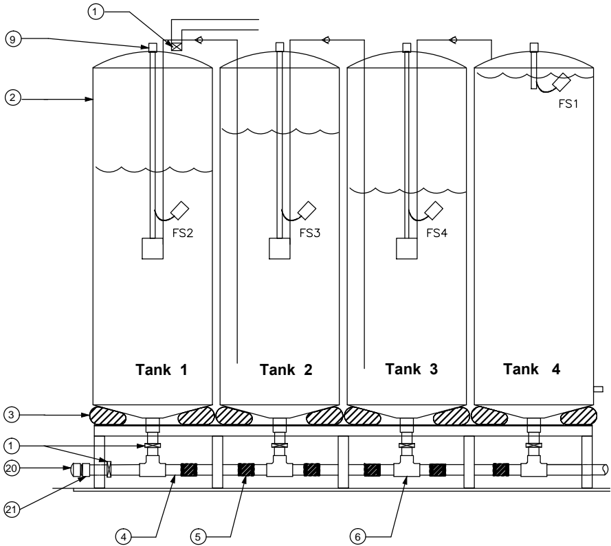
Elevation Tanks 1,2,3,4
