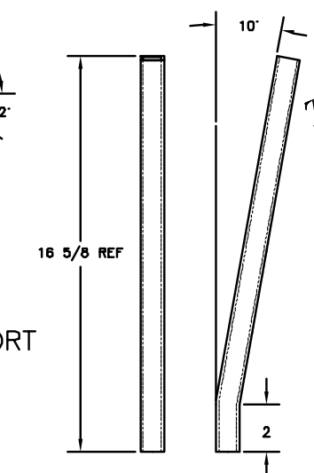
12 CENTER SUPPORT SCALE X2
