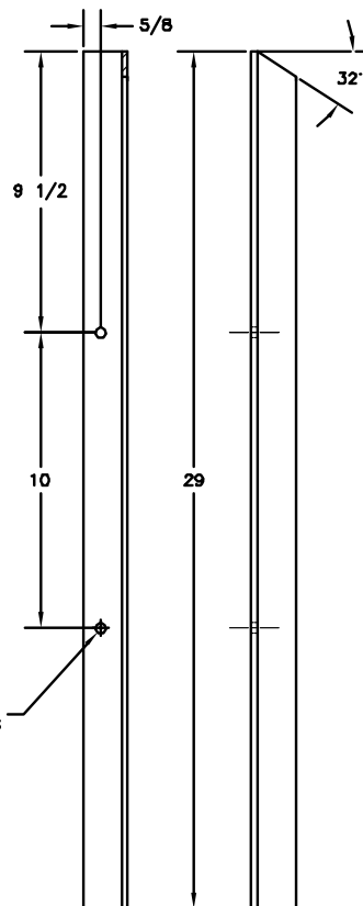
10 POST RAIL SCALE X2
