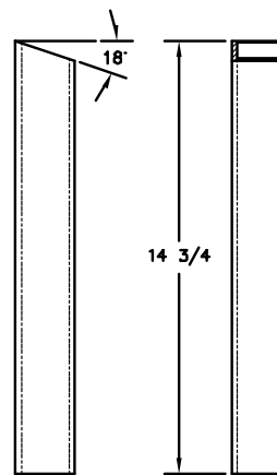
4 BACK LEG SCALE X2
