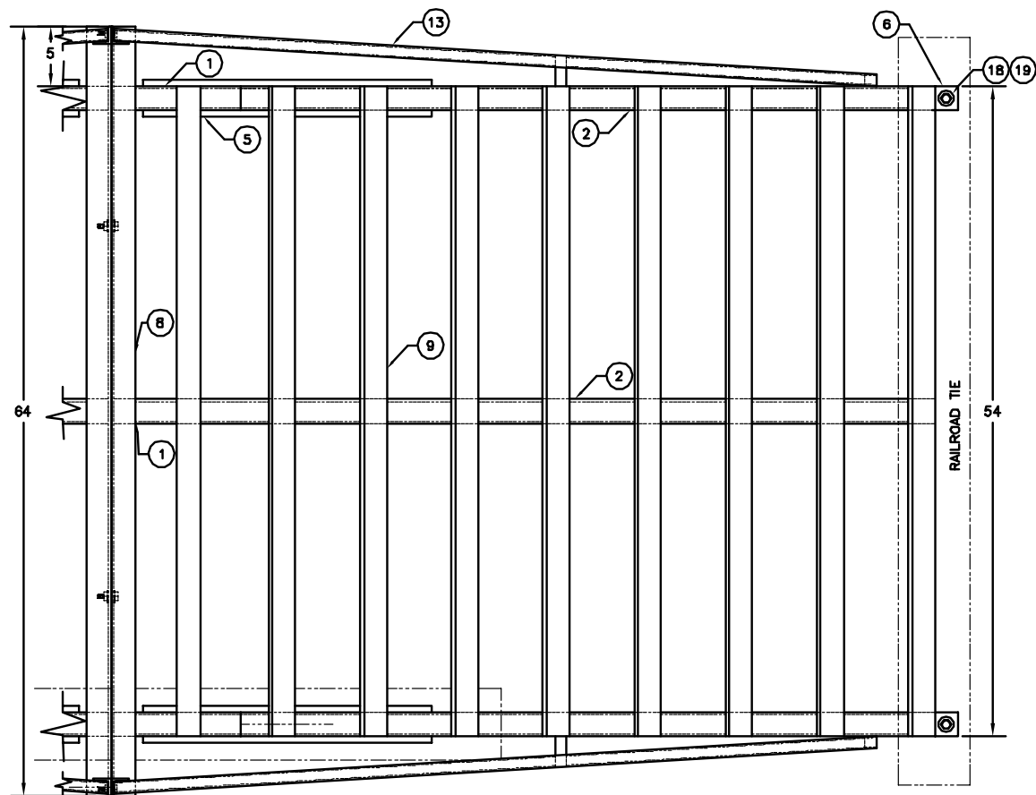
4 BACK LEG SCALE X2
