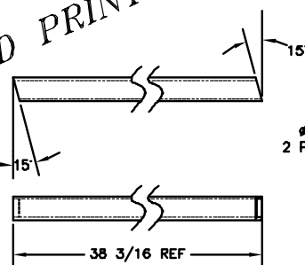
14 CROSS SUPPORT SCALE X2
