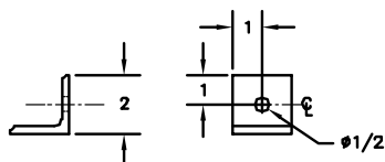
6 TAB SCALE X2
