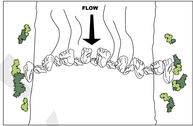
Figure 57—Grade stabilizer is placed at grade to prevent channel incision.
