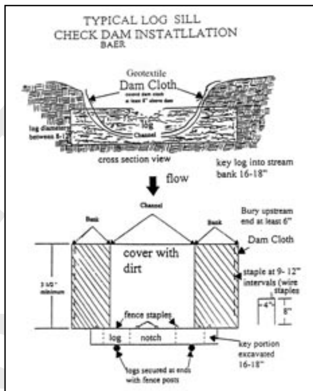
Figure 48—Typical log checkdam structure.
