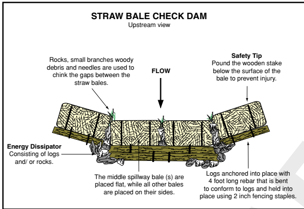
Figure 51—Strawbale checkdam (upstream view)
