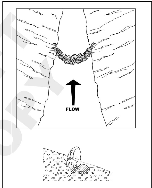
Figure 59—Stream grade can be adjusted and maintained by careful placement of boulders.
