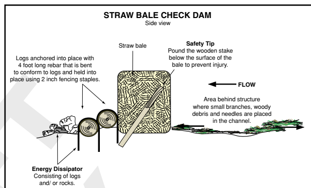
Figure 49—Strawbale checkdam (sideview)
