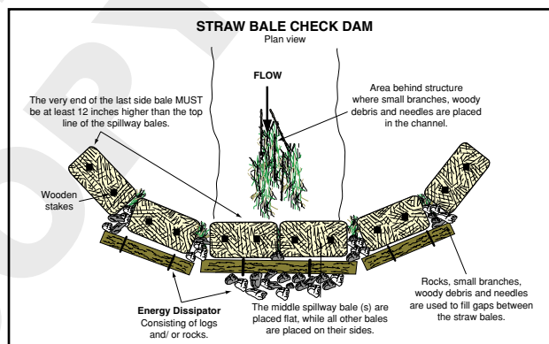
Figure 50—Strawbale checkdam (planview)
