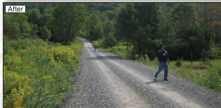
Figure 2.17 and 2.18—This roadway cuts across a flood plain wetland. A 300-foot-long French mattress was used to provide relief for wetland flows while providing a stable road base and preventing beavers from damming the nearby stream pipe.
