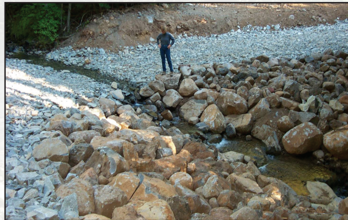
Figure 6.9—Boulder ford on Stanislaus National Forest in California has had no maintenance since construction in 1997.
