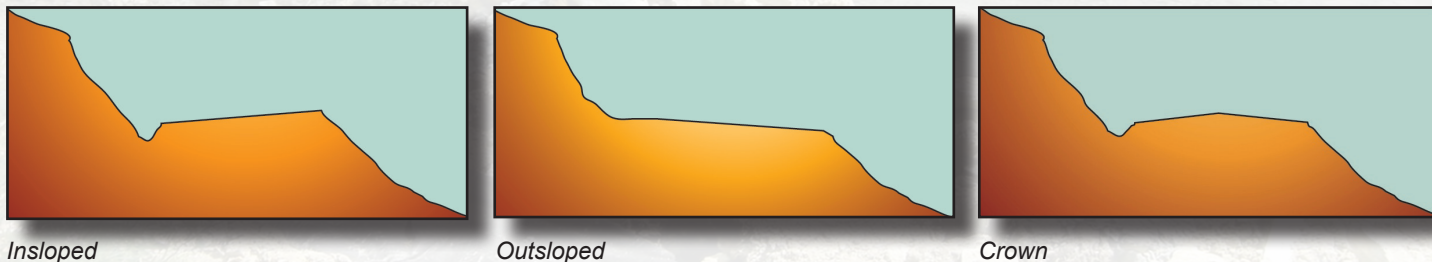
Figures 3.2—Road surface templates.
