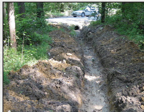
Figure 5.5—Traditional deep pipe. It has a long outlet trench requiring continual maintenance.
