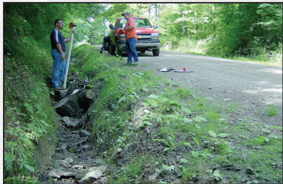
Figure 4.4—This eroded ditch is a symptom. The problem is excessive water volume for this road gradient and soil, and must be managed upslope.
