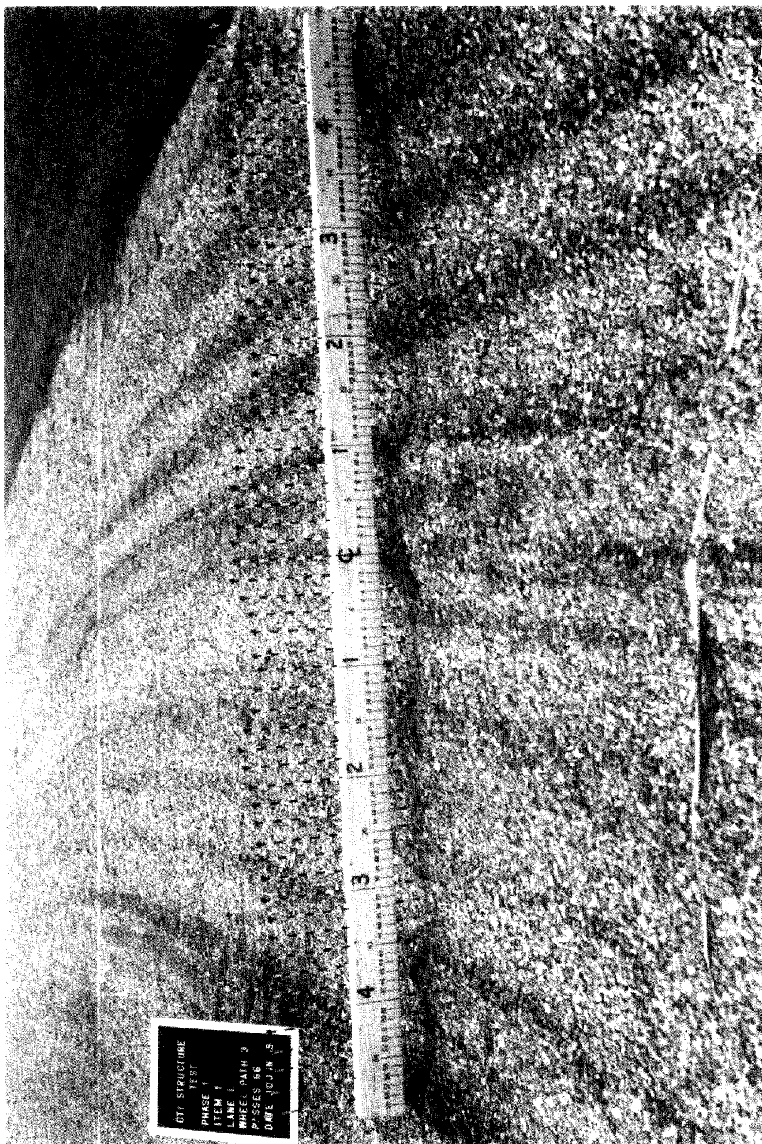
Photo 42. Item 1, low-pressure tire lane, failure after 66 passes
