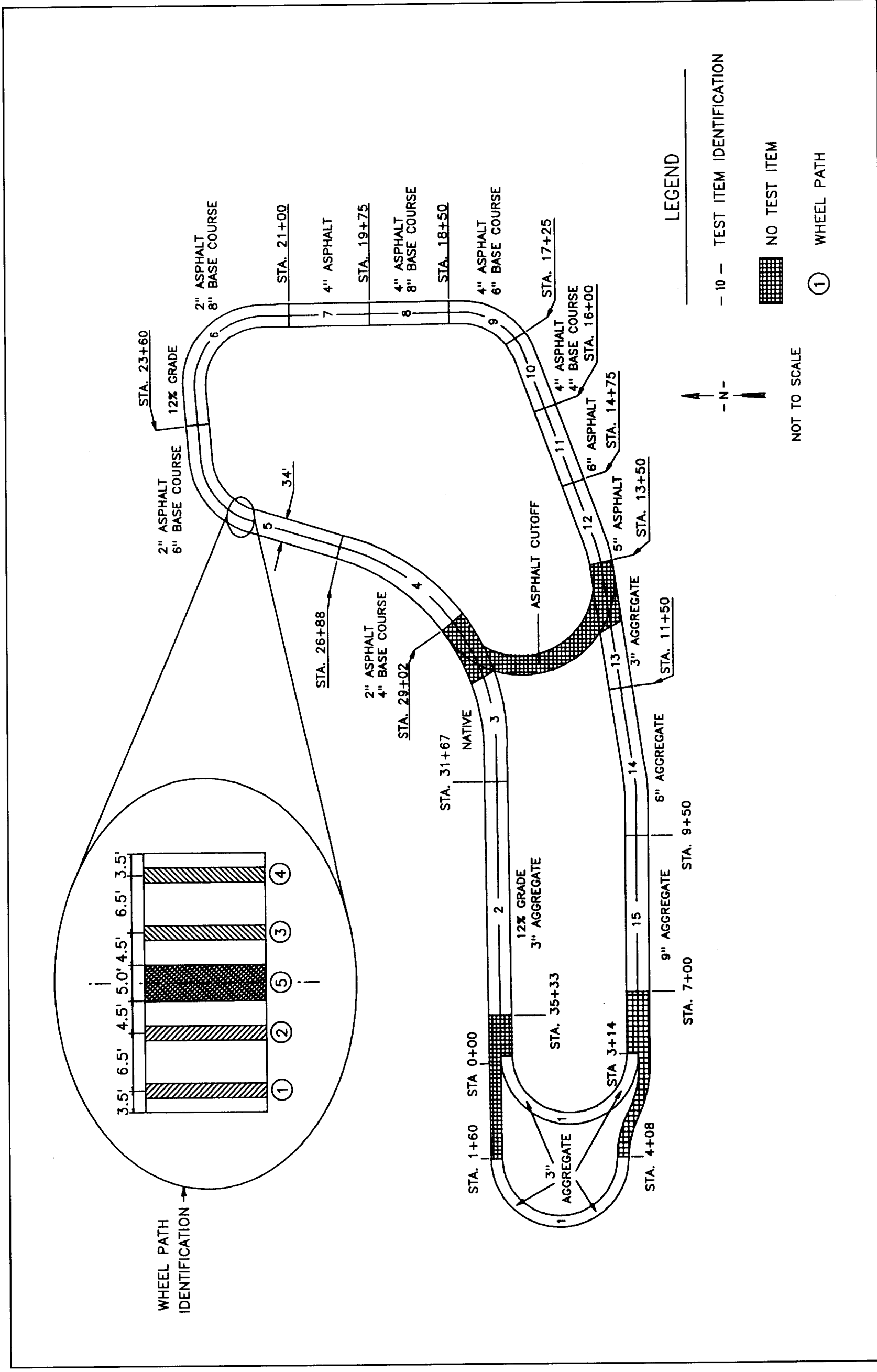
Figure 1. Plan view of test road
