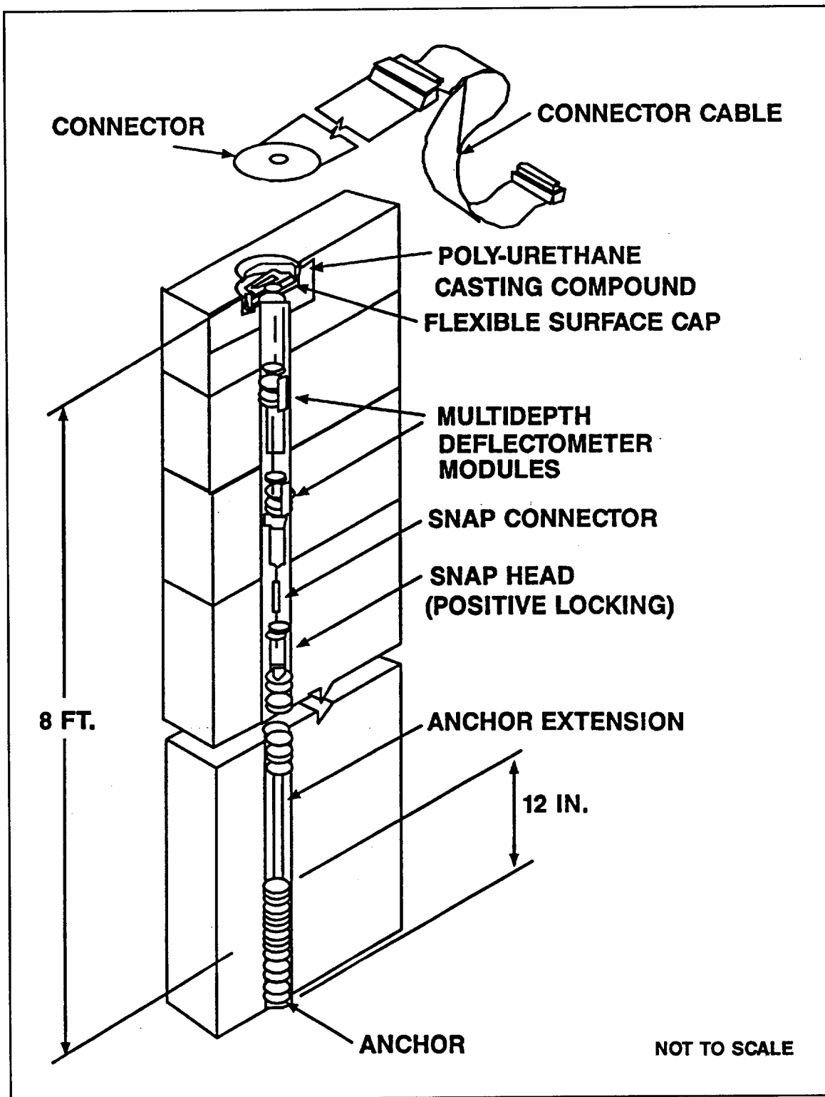
Figure 9. Typical cross section of a MDD after installation
