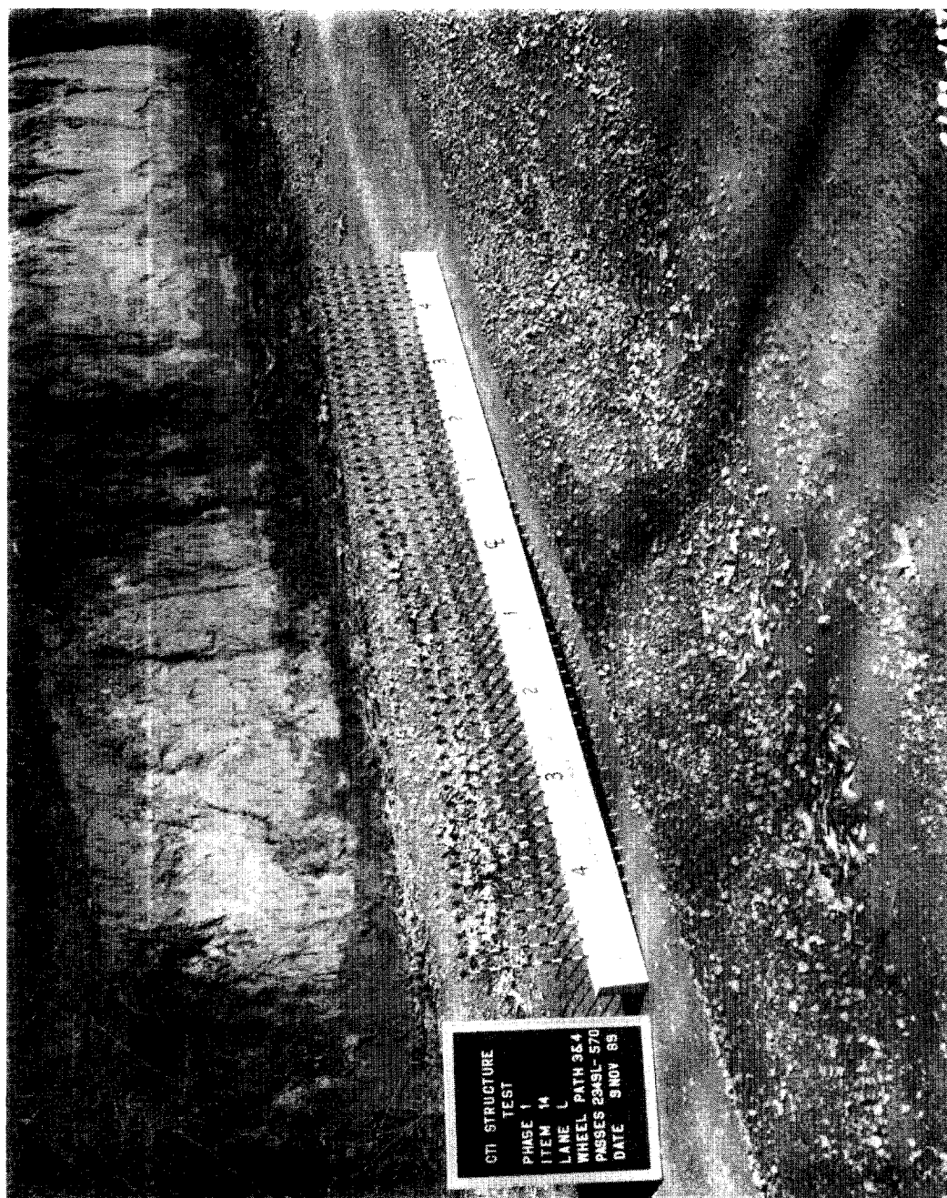
Photo 64. Item 14, low-pressure tire lane, low-severity depression after 570 passes during the induced failure plan
