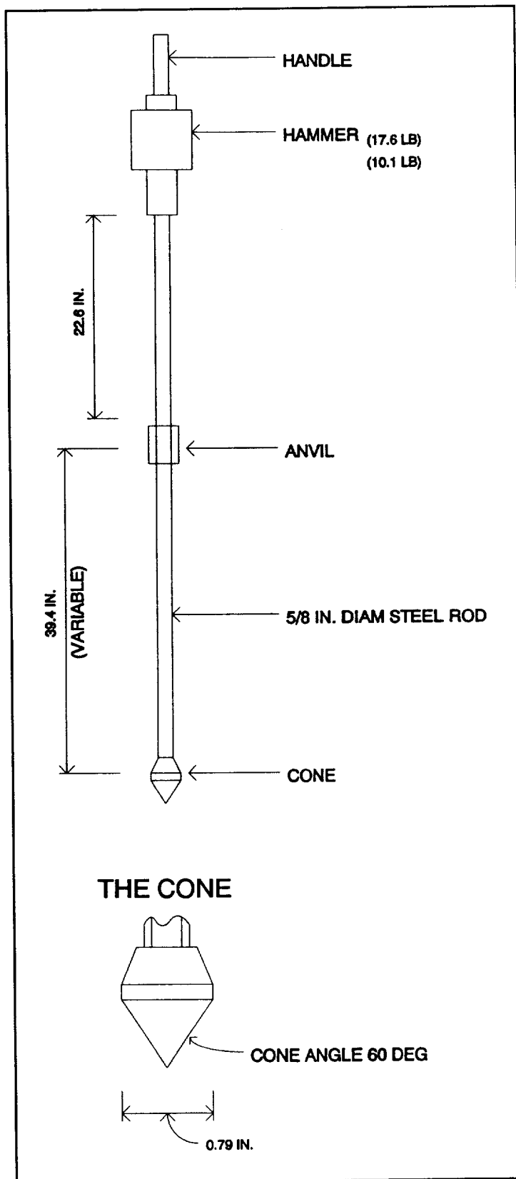
Figure 16. Plan view of dynamic cone penetrometer
