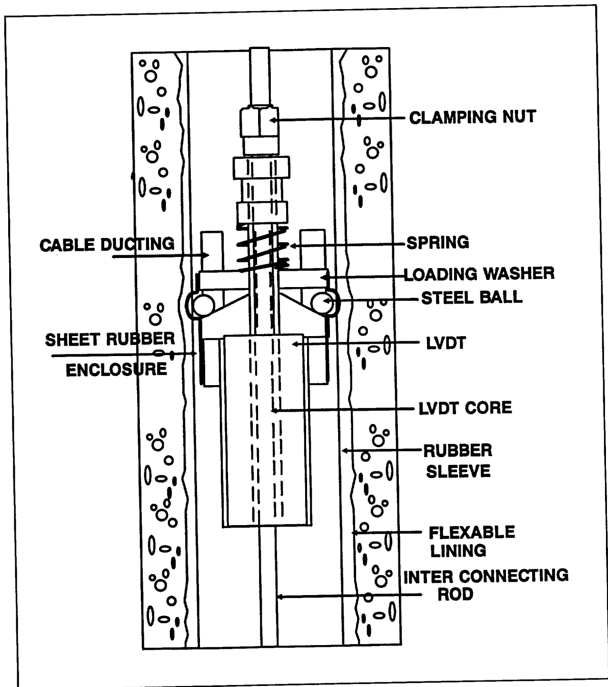
Figure 8. Components of an MDD module
