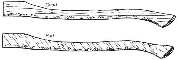
The grain of ax handles should run parallel to the wedge slot.
