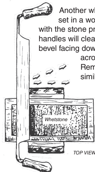
Sharpening a drawknife using a stone set in a wood block.
