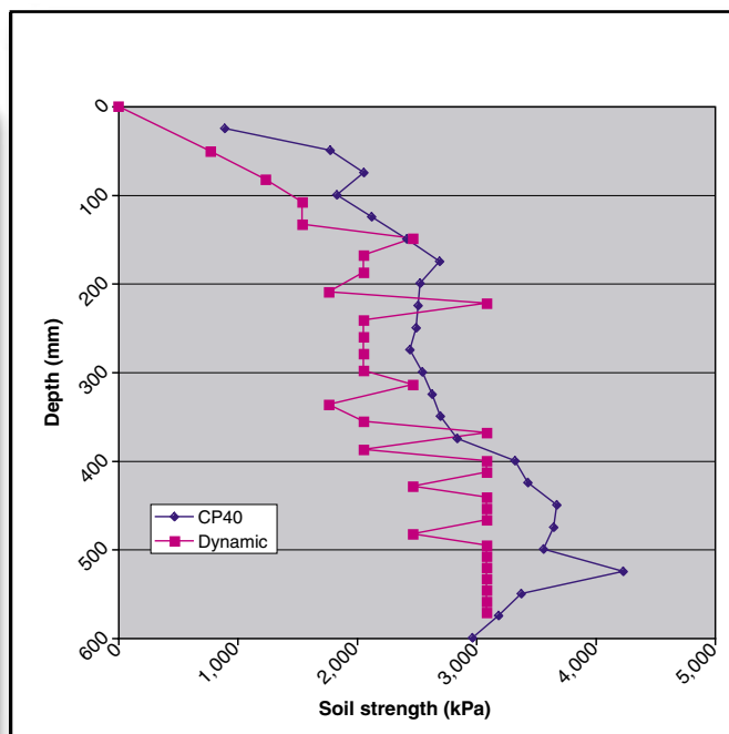
Figure 13—Relative differences between a hand-held electronic cone penetrometer and a dynamic cone penetrometer.
