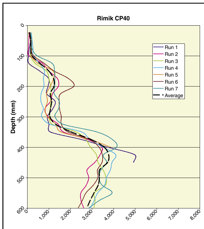
Figure 6—Repetition testing of the Rimik CP40 shows the unit's consistency in documenting soil strength at various depths. Even though the runs were conducted about 300 mm from each other, some variation in readings can be expected because of differences in ground conditions, equipment tracks, and operator inconsistency. The Rimik CP40 displays metric units.
