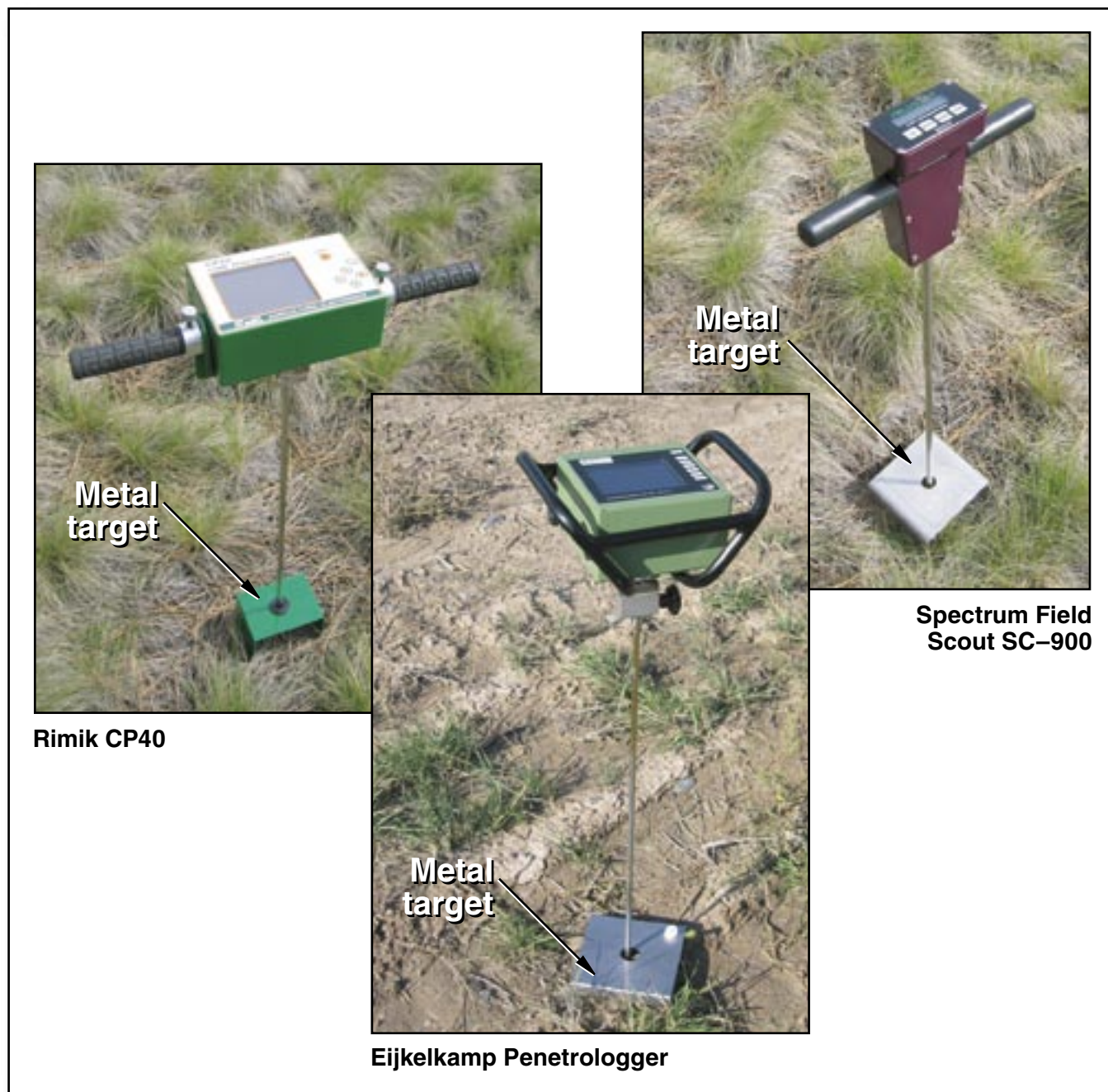
Figure 3—The three hand-held electronic cone penetrometers tested by MTDC were the Rimik CP40 (left); the Eijkelkamp Penetrologger (center); and the Spectrum Field Scout SC-900 (right).
