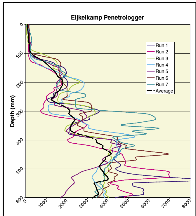
Figure 7—Repetition testing of the Eijkelkamp Penetrologger. The first 100 mm of soil was weak because of recent tillage in the test field. The Eijkelkamp Penetrologger displays metric units.
