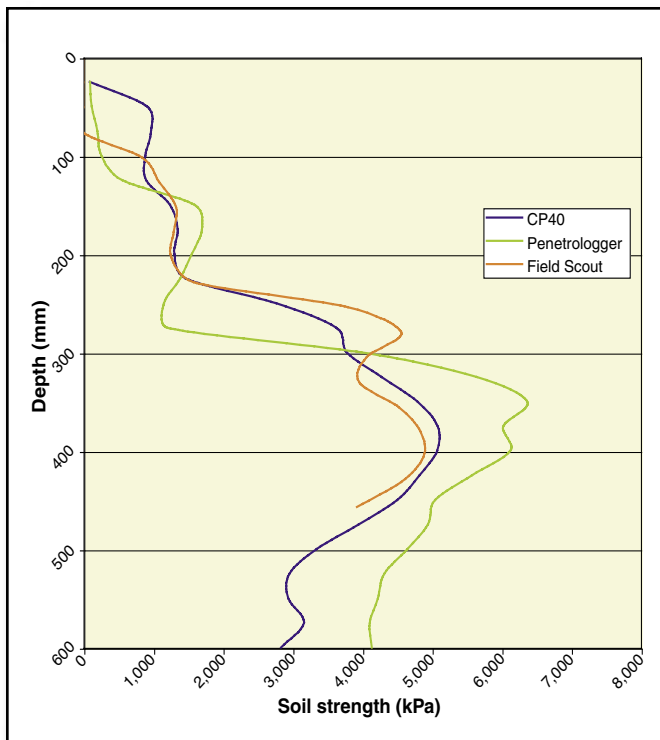
Figure 9—In the side-by-side comparison test, all three penetrometers were reasonably consistent. Probes were about 300 mm from each other.
