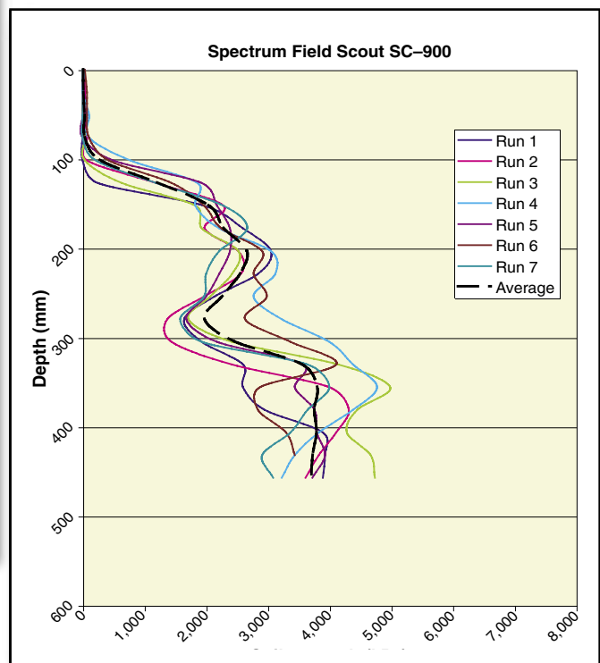
Figure 8—Repetition testing of the Spectrum Field Scout SC-900. The SC-900 outputs English or metric units.
