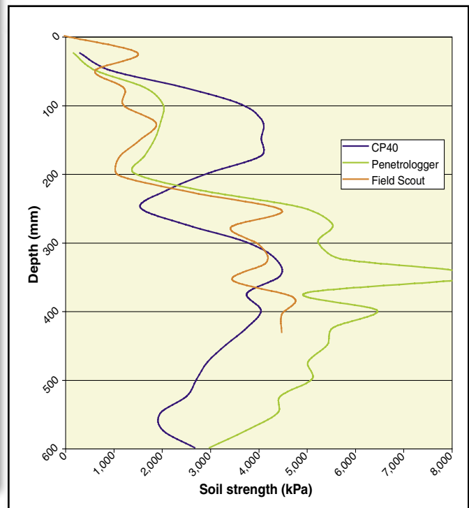
Figure 11—This test shows some variation between the three units in the side-by-side test. The wild jump in soil strength on the Eijkelkamp Penetrologger was caused by a rock or very hard object at a depth of about 350 mm.
