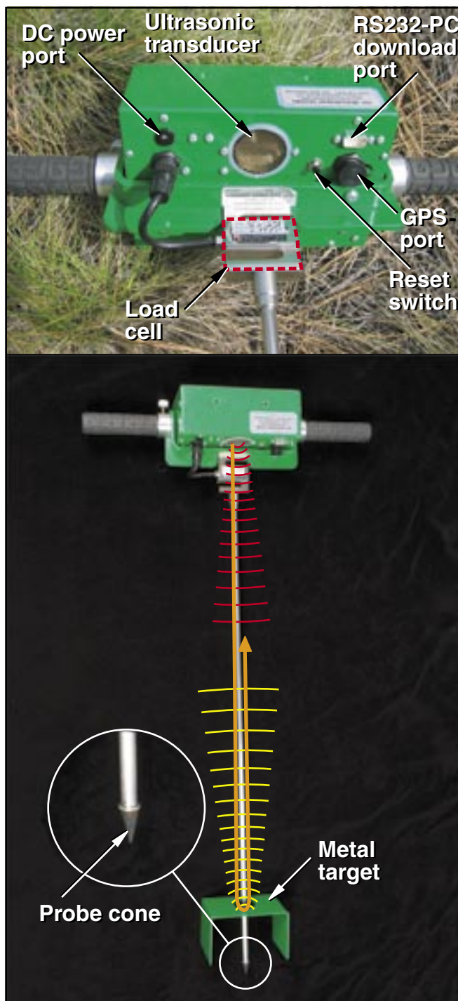
Figures 4—The operating components of a typical hand-held cone penetrometer. The metal target bounces a signal back to the transducer, allowing the penetrometer to calculate the probe's depth. These photos show the Rimik CP40.
