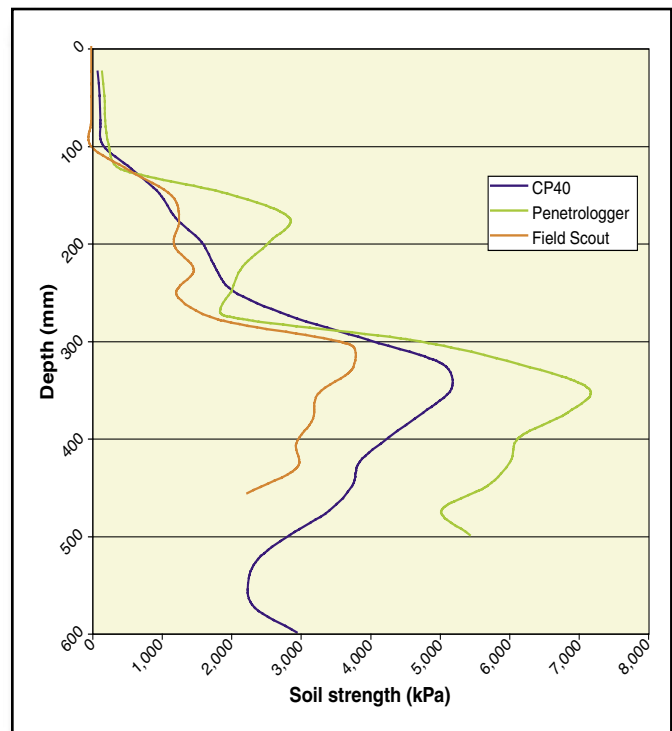
Figure 10—The results from this comparison test show less consistency, probably because of variation in ground conditions, equipment tracks, or operator inconsistency.
