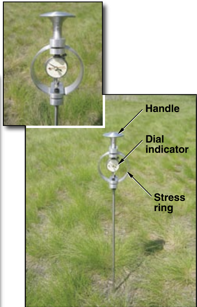
Figure 2—Mechanical cone penetrometers have been used for decades. A dial indicator mounted inside a metal stress ring shows the force exerted on the handle of this vintage penetrometer.
