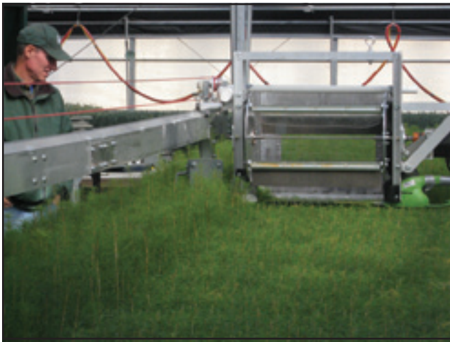
Figure 1b—The MTDC prototype top pruner in use at the Lucky Peak Nursery.
