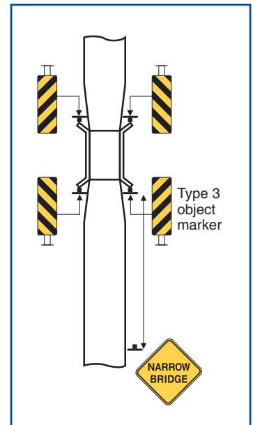
Single-Lane Road With Narrow Bridge
