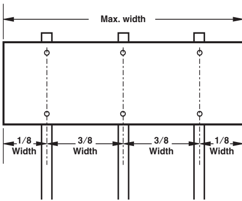
Three-Post Spacing* (Nonbreakaway installation)
