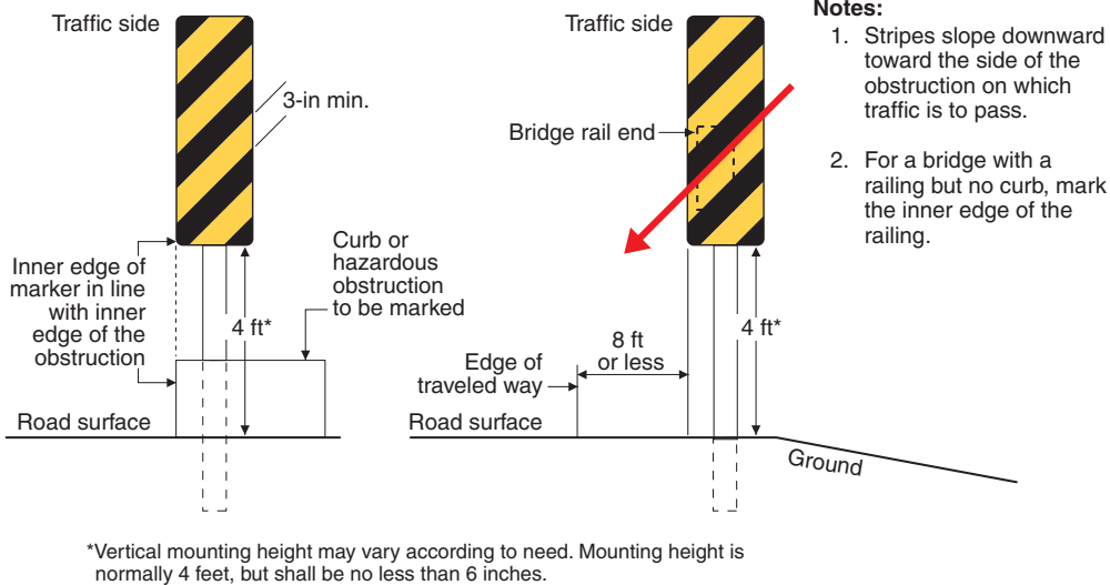
Placement of Type 3 Object Markers
