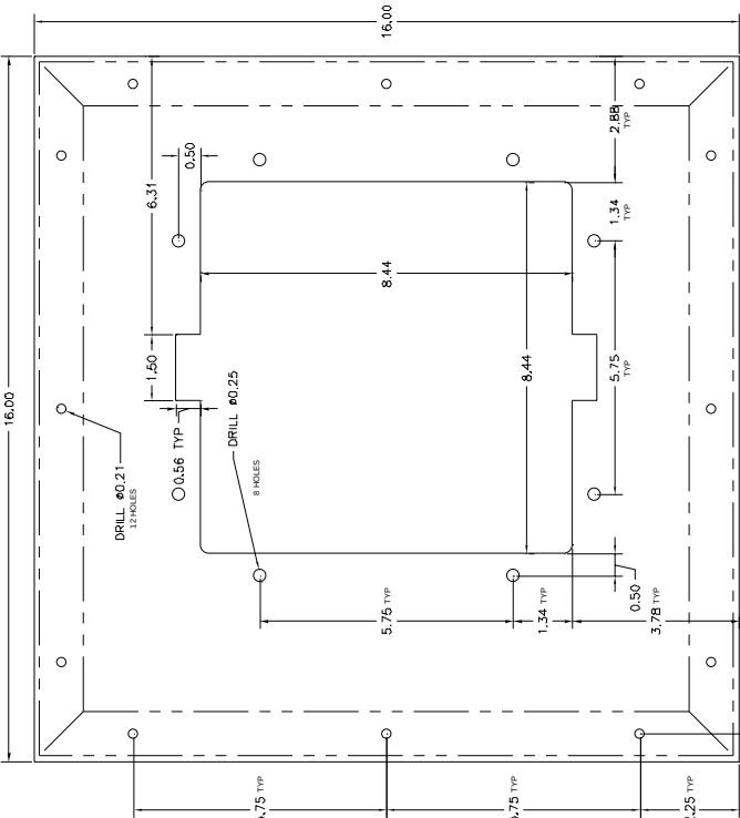
73 TOP COVER
